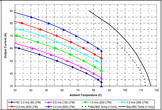
Maximum output current vs. ambient temperature at nominal input voltage for airflow rates natural convection (0.3m/s) to 3.0m/s with airflow from pin 3 to pin 1.
