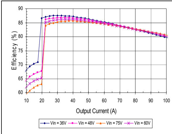
Efficiency vs. Input Voltage at Ta=25C, (use socket)
