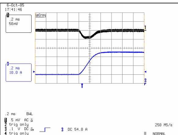
Load Transient Response. Load Step from 50% to 75% of Full Load with di/dt= 0.1A/uS. Ch. 1: Vo Ch. 3: Io
