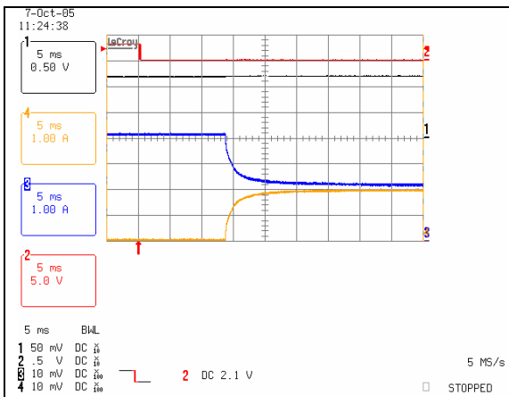
Start-up with Back-biased Voltage (1.2V) and 4A Load. Ch. 1: Vo Ch. 2: ON/OFF Ch. 3: Io1 Ch. 4: Io2
