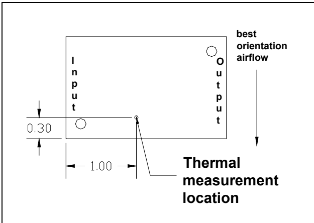
Thermal measurement location – top view
