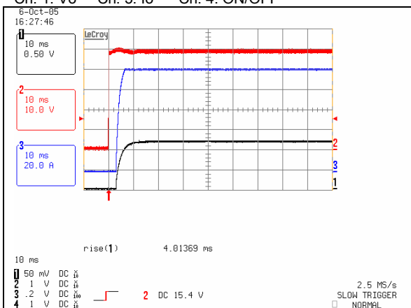
Start-up from Input Voltage Application at Full Load. Ch. 1: Vo Ch. 2: Vin Ch. 3: Io
