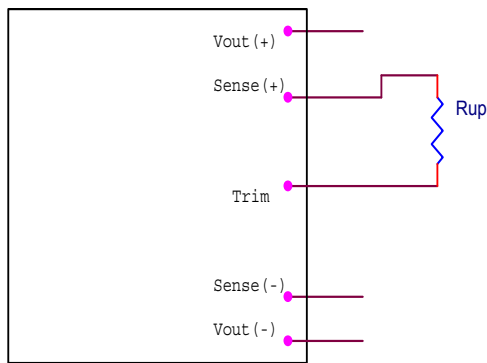
Circuit to increase output voltage
