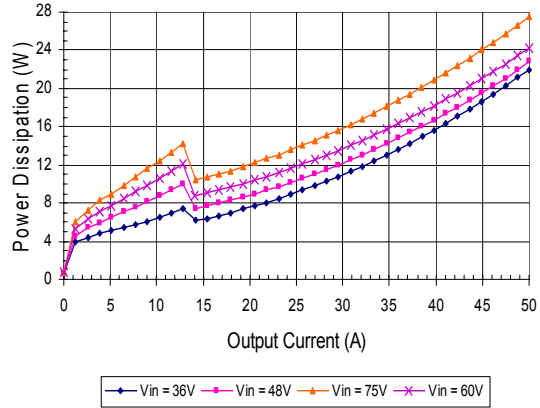
Power Dissipation vs. Input Voltage at Ta=25C
