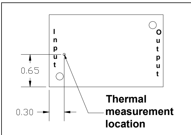
Thermal measurement location on baseplate – top view
