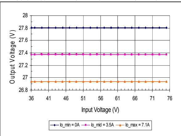
Typical Output Voltage vs. Vin at Ta=25C.
