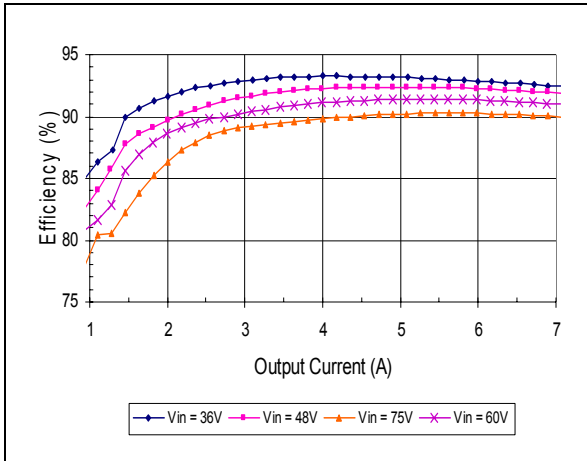
Efficiency vs. Vin at Ta=25°C, No Heat Sink
