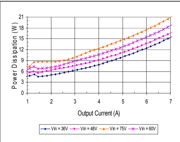
Power Dissipation vs. Vin at Ta=25°C, No Heat Sink
