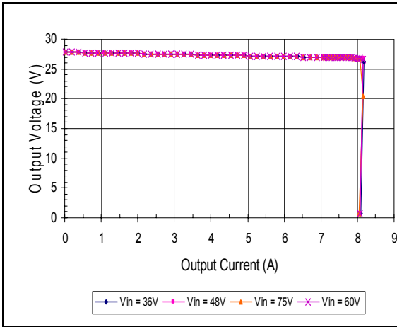
Output Current Limit Characteristics vs. Vin at Ta=25C.
