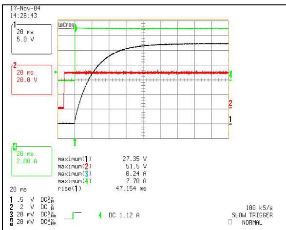
Start-up constant current load from Vin Application Ch. 1: Vo Ch. 2: Vin Ch. 4: Io
