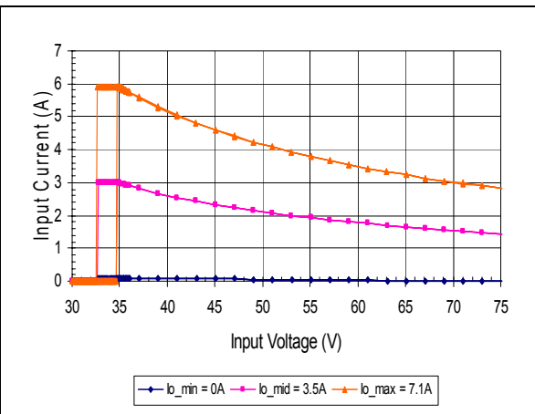
Typical Input Current vs. Vin Characteristics
