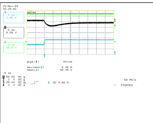
Transient Response. Load Step from 50% to 75% of Full Load with di/dt= 0.1A/uS. Ch. 1: Vo Ch. 3: Io
