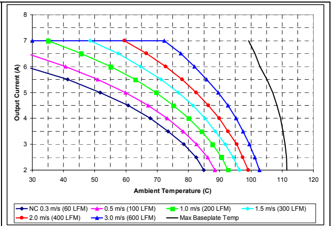
Maximum output current vs. ambient temperature at nominal input voltage for airflow rates of 0.3m/s to 3.0m/s with airflow from pin 1 to pin 8.
