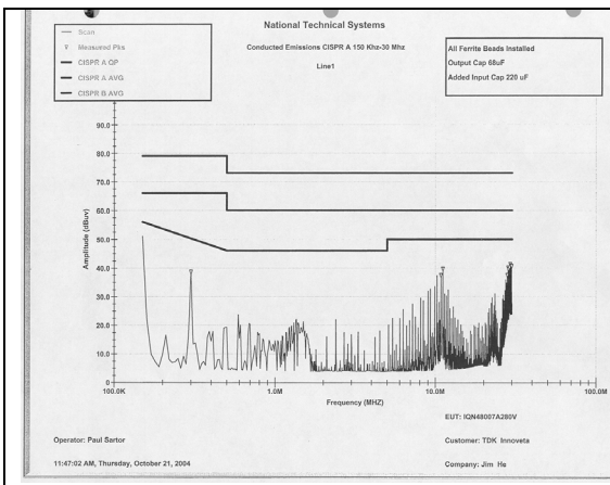
Conducted Emission with CISPR Class B
