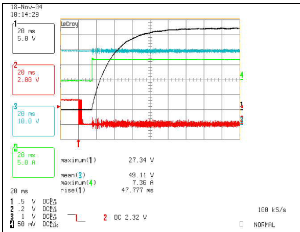
Start-up constant current load from on/off switch, 48V Vin Ch. 1: Vo Ch. 2: on/off Ch. 3: Vin Ch. 4: Io
