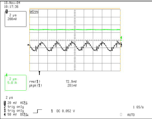
Typical Output Ripple at 48V Input and Full Load. Cext=440uF. Ch. 1: Vo Ch. 4: Io
