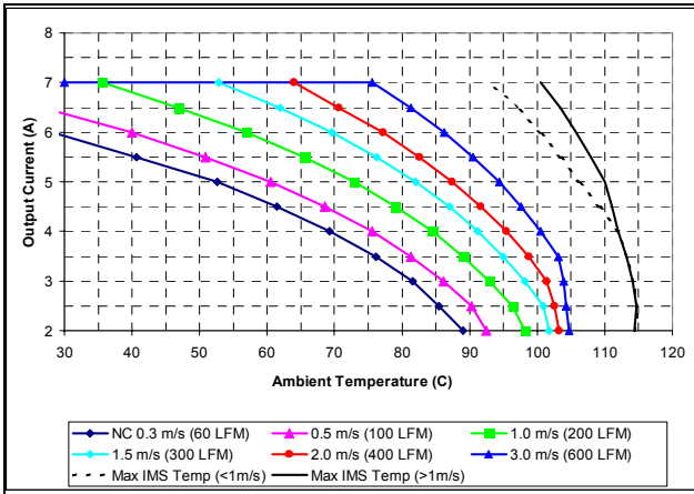
Maximum output current vs. ambient temperature at nominal input voltage for airflow rates of 0.3m/s to 3.0m/s with airflow from pin 3 to pin 1 (best orientation).
