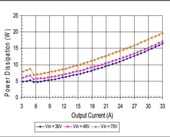
Power Dissipation vs. Input Voltage at Ta=25°C, No Heat Sink
