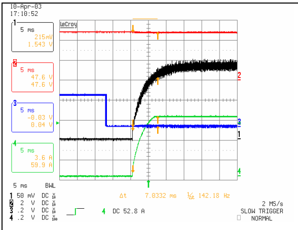
Start-up on on/off Switch at 48V input and Full Load. Ch. 1: Vo Ch. 2: Vin Ch. 3: ON/OFF Ch. 4: Io
