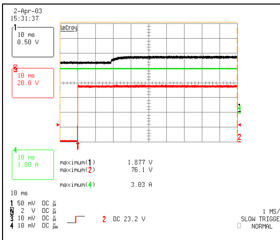
Start-up with Back-biased Voltage (1.7V) and 3A Load. Ch. 1: Vo Ch. 2: Vin Ch. 4: Io
