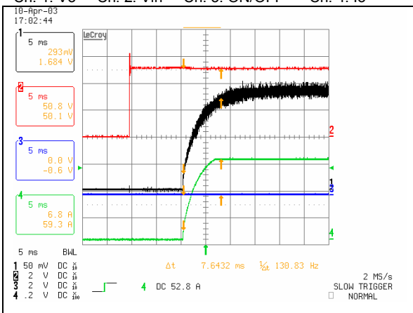
Start-up from Input Voltage Application at Full Load. Ch. 1: Vo Ch. 2: Vin Ch. 3: ON/OFF Ch. 4: Io
