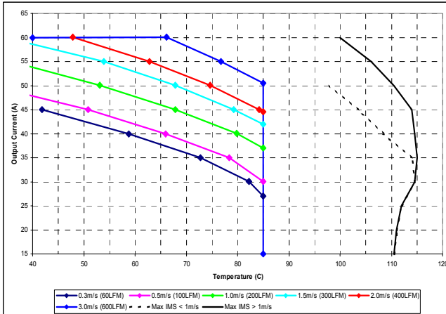
Maximum output current vs. ambient temperature at nominal input voltage for airflow rates natural convection (0.3m/s) to 3.0m/s with airflow from pin 3 to pin 1 (best orientation).
