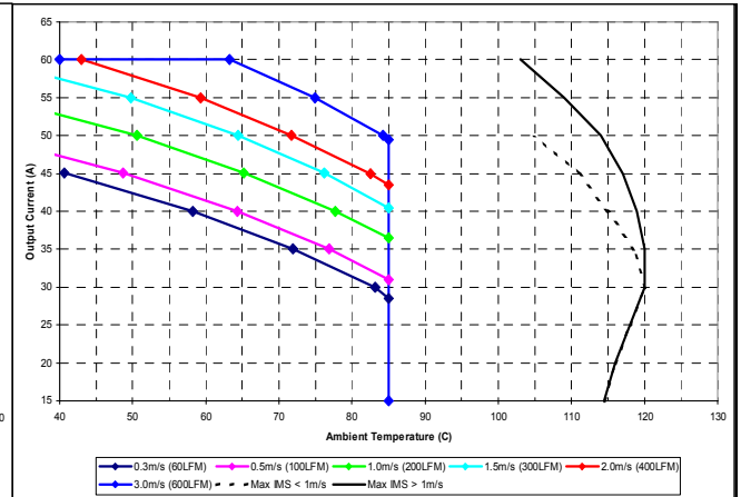
Maximum output current vs. ambient temperature at nominal input voltage for airflow rates natural convection (0.3m/s) to 3.0m/s with airflow from pin 1 to pin 3.
