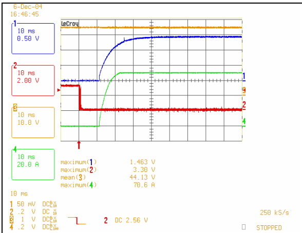
Start-up from on/off Switch, 48Vin, Full Load, Cext,min. Ch. 1: Vo Ch. 2: ON/OFF Ch. 3: Vin Ch. 4: Io
