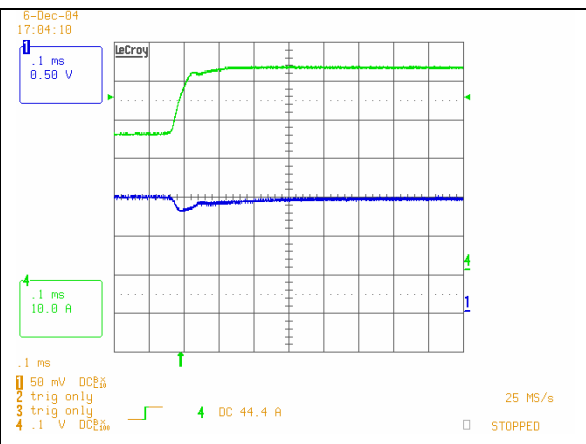
Load Transient Response. Load Step from 50% to 75% of Full Load with di/dt= 0.1A/uS. Ch. 1: Vo Ch. 4: Io
