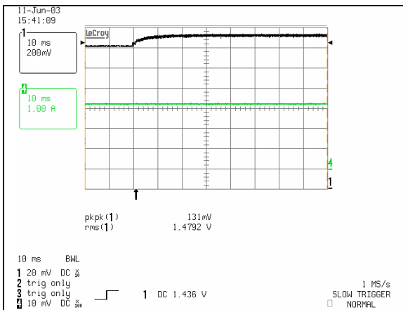
Start-up with Back-biased Voltage (1.4V) and 3A Load. Ch. 1: Vo Ch. 4: Io
