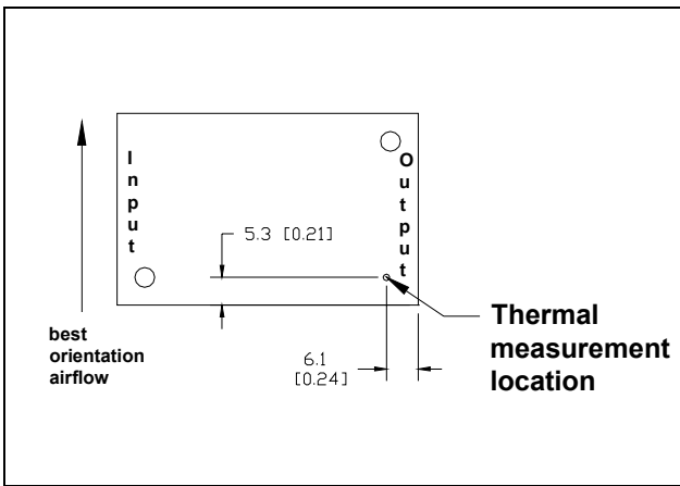
Thermal measurement location – top view
