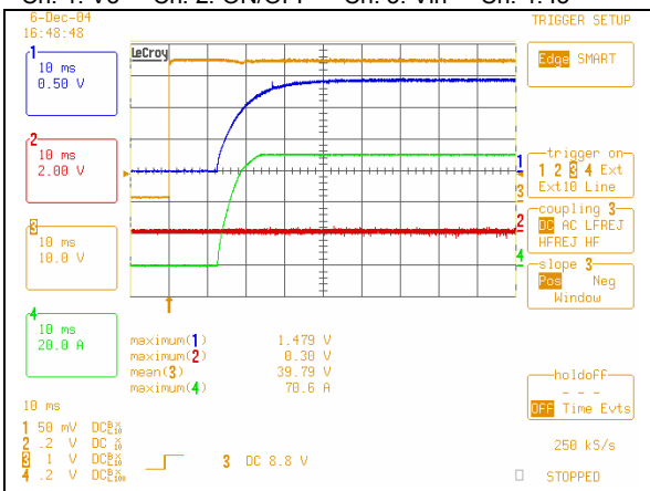
Start-up from Nominal Vin, Full Load, and Cext, min. Ch. 1: Vo Ch. 2: ON/OFF Ch. 3: Vin Ch. 4: Io
