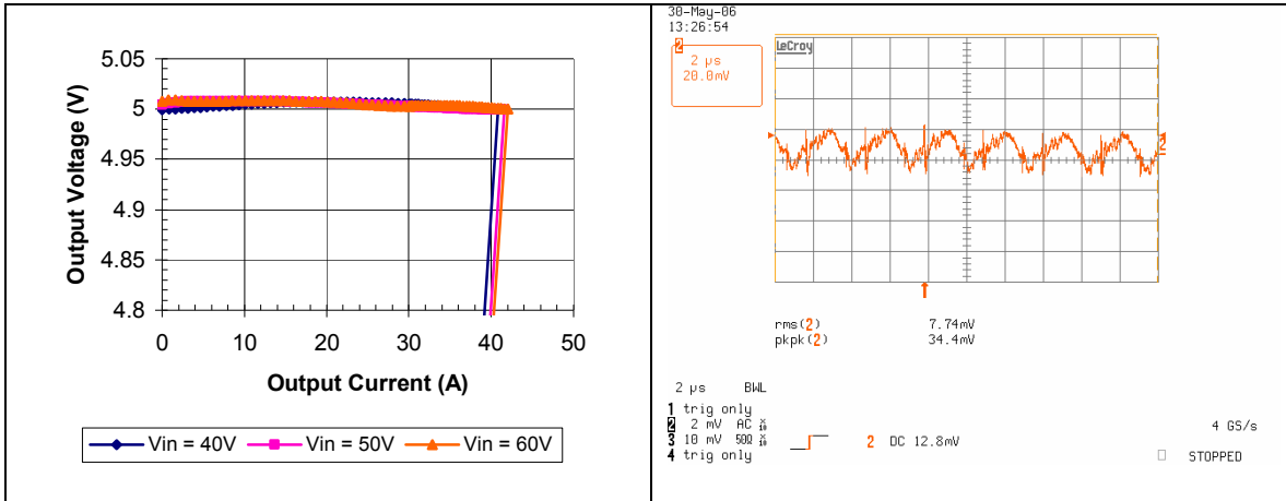
iQE48030A050V-001 Typical Output Current Limit Characteristics vs. Input Voltage at Ta=25 degrees.
