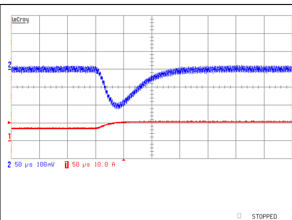
iQE48014A080V-001 Typical transient response. Output voltage response to load step from 50% to 75% of full load with output current slew rate of 0.1A/μS.
