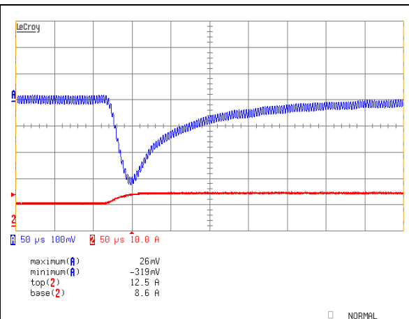
iQE48017A120V-001 Typical transient response. Output voltage response to load step from 50% to 75% of full load with output current slew rate of 0.1A/μS.
