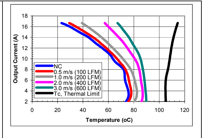
iQE48017A120V-001 maximum output current vs. ambient temperature at nominal input voltage for airflow rates natural convection (60lfm) to 600lfm with airflow from pin 1 to pin 3
