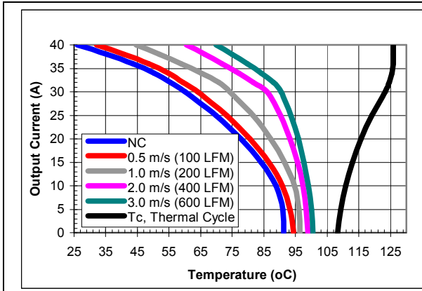
iQE48040A033V-001 maximum output current vs. ambient temperature at nominal input voltage for airflow rates natural convection (60lfm) to 600lfm with airflow from pin 3 to pin 1 (best orientation).
