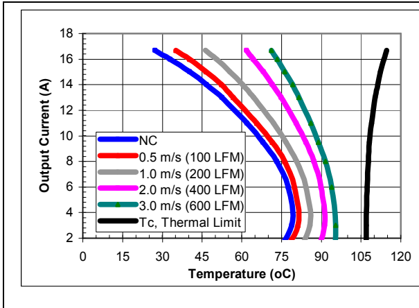
iQE48017A120V-001 maximum output current vs. ambient temperature at nominal input voltage for airflow rates natural convection (60lfm) to 600lfm with airflow from pin 3 to pin 1 (best orientation).
