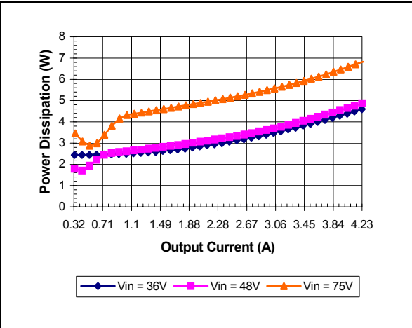
iQB48004A120V-000 Typical Power Dissipation vs. Input Voltage at Ta=25 degrees
