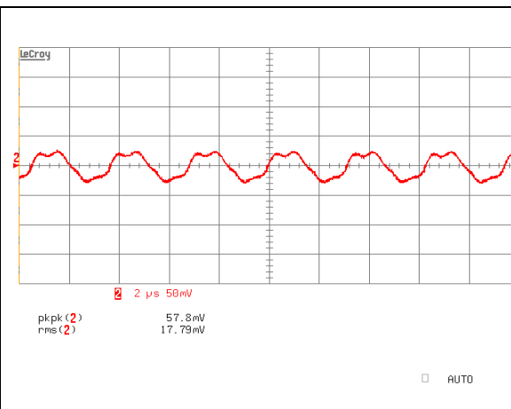
iQB48004A120V-000 Typical Output Ripple at nominal Input voltage and full load at Ta=25 degrees
