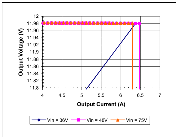
iQB48004A120V-000 Typical Output Current Limit Characteristics vs. Input Voltage at Ta=25 degrees.
