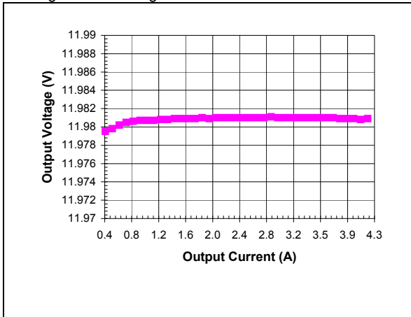
iQB48004A120V-000 Typical Output Voltage vs. Load Current at Ta = 25 degrees
