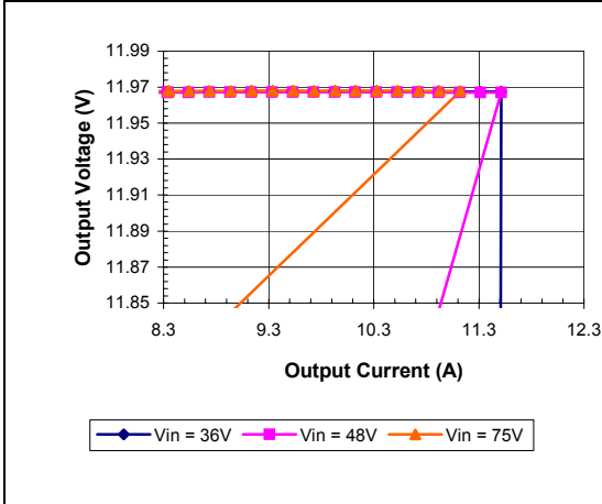
iQB48008A120V-000 Typical Output Current Limit Characteristics vs. Input Voltage at Ta=25 degrees.
