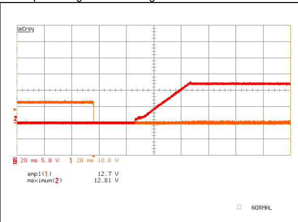
iQB48008A120V-001 Typical startup characteristic from on/off at full load. Upper trace – output voltage, lower trace – on/off signal
