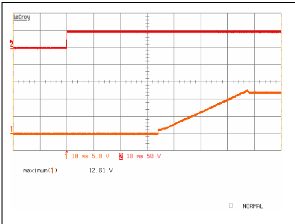
iQB48012A120V-000 Typical startup characteristic from input voltage application at full load. Upper trace - input voltage, lower trace – output voltage
