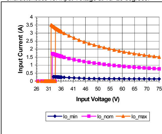
iQB48008A120V-000 Typical Input Current vs. Input Voltage Characteristics
