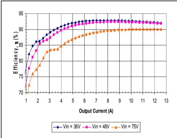
iQB48012A120V-000 Typical Efficiency vs. Input Voltage at Ta=25 degrees.
