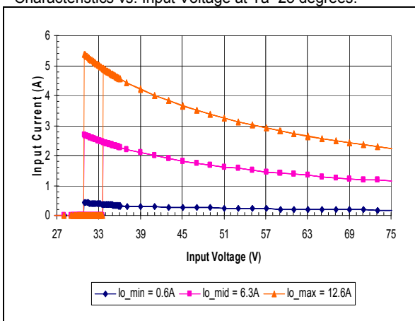
iQB48012A120V-000 Typical Input Current vs. Input Voltage Characteristics
