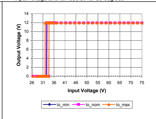
iQB48008A120V-000 Typical Output Voltage vs. Input Voltage Characteristics
