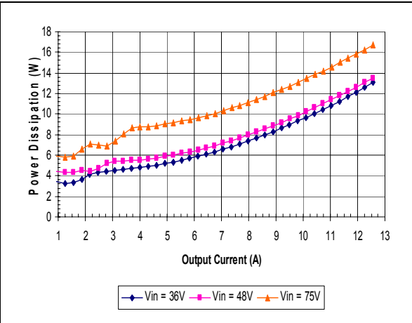
iQB48012A120V-000 Typical Power Dissipation vs. Input Voltage at Ta=25 degrees
