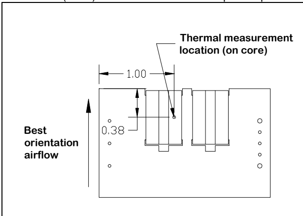
iQB48012A120V-000 thermal measurement location – top view
