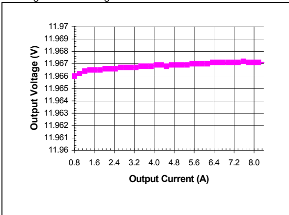
iQB48008A120V-000 Typical Output Voltage vs. Load Current at Ta = 25 degrees
