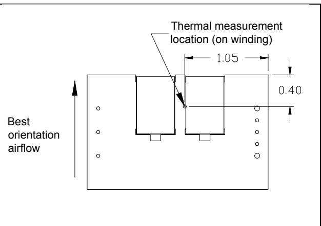
iQB48004A120V-000 thermal measurement location – top view
