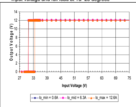
iQB48012A120V-000 Typical Output Voltage vs. Input Voltage Characteristics
