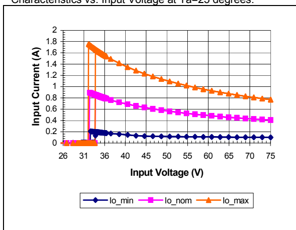
iQB48004A120V-000 Typical Input Current vs. Input Voltage Characteristics
