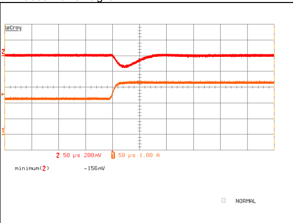
iQB48004A120V-000 Typical transient response. Output voltage response to load step from 50% to 75% of full load with output current slew rate of 0.1A/ \mu S.
