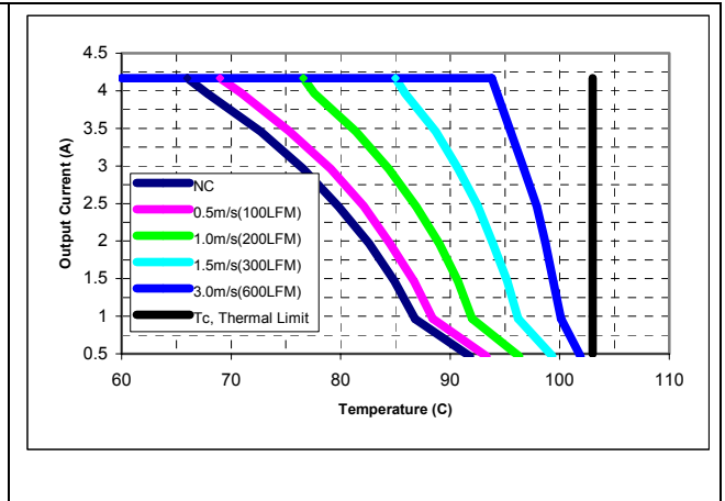
iQB48004A120V-000 maximum output current vs. ambient temperature at nominal input voltage for airflow rates natural convection (60lfm) to 600lfm with airflow from pin 1 to pin 3 (worst orientation)
