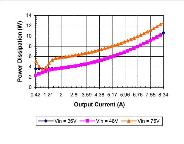
iQB48008A120V-000 Typical Power Dissipation vs. Input Voltage at Ta=25 degrees
