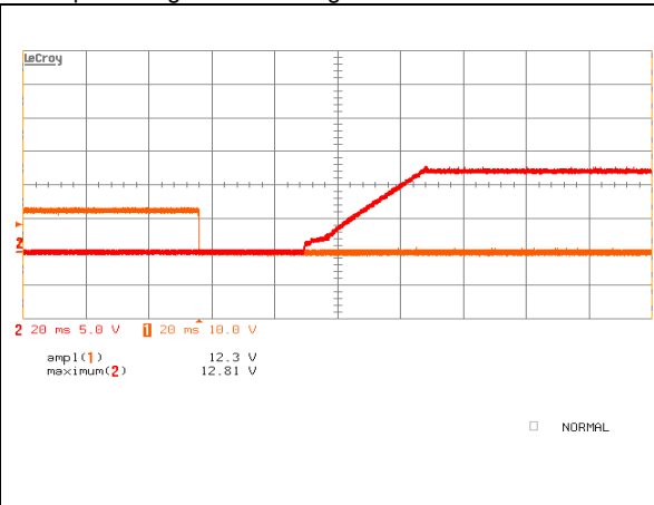
iQB48004A120V-001 Typical startup characteristic from on/off at full load. Upper trace – output voltage, lower trace – on/off signal
