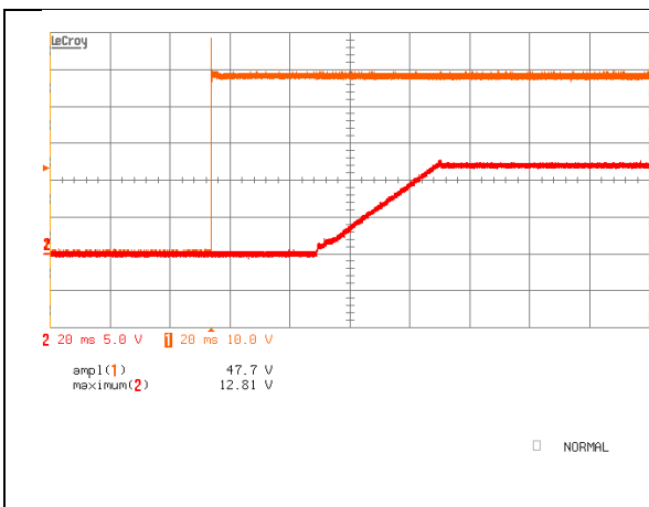
iQB48008A120V-000 Typical startup characteristic from input voltage application at full load. Upper trace - input voltage, lower trace – output voltage
