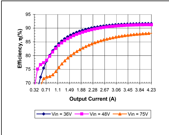
iQB48004A120V-000 Typical Efficiency vs. Input Voltage at Ta=25 degrees.
