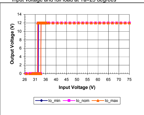
iQB48004A120V-000 Typical Output Voltage vs. Input Voltage Characteristics
