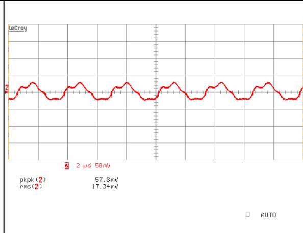
iQB48008A120V-000 Typical Output Ripple at nominal Input voltage and full load at Ta=25 degrees
