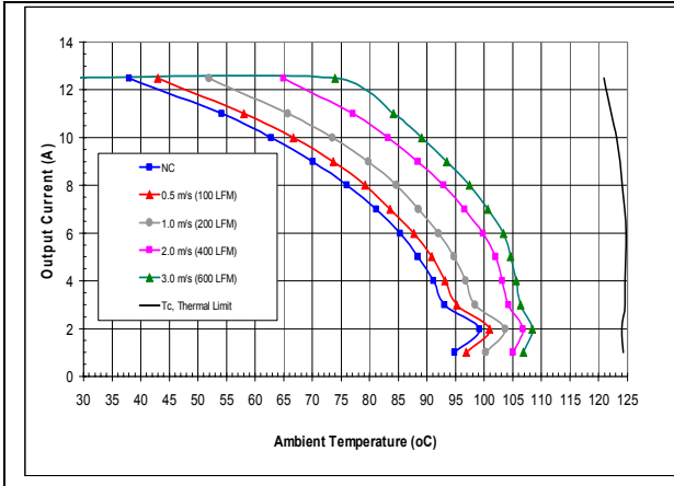
iQB48012A120V-000 maximum output current vs. ambient temperature at nominal input voltage for airflow rates natural convection (60lfm) to 600lfm with airflow from pin 3 to pin 1.
