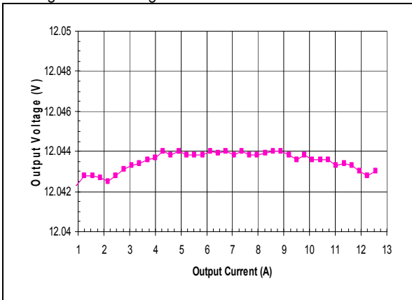
iQB48012A120V-000 Typical Output Voltage vs. Load Current at Ta = 25 degrees
