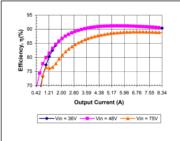
iQB48008A120V-000 Typical Efficiency vs. Input Voltage at Ta=25 degrees.
