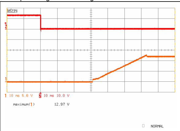
iQB48012A120V-001 Typical startup characteristic from on/off at full load. Lower trace – output voltage, upper trace – on/off signal
