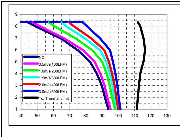
iQB48008A120V-000 maximum output current vs. ambient temperature at nominal input voltage for airflow rates natural convection (60lfm) to 600lfm with airflow from pin 3 to pin 1 (best orientation).
