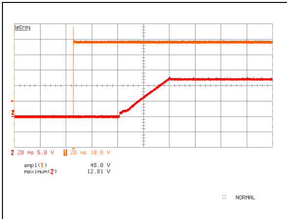
iQB48004A120V-000 Typical startup characteristic from input voltage application at full load. Upper trace - input voltage, lower trace – output voltage
