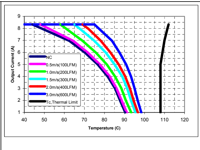
iQB48008A120V-000 maximum output current vs. ambient temperature at nominal input voltage for airflow rates natural convection (60lfm) to 600lfm with airflow from pin 1 to pin 3 (worst orientation)
