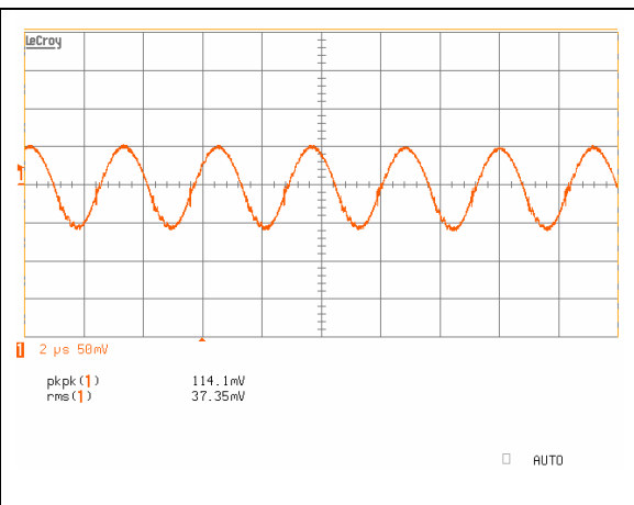
iQB48012A120V-000 Typical Output Ripple at nominal Input voltage and full load at Ta=25 degrees
