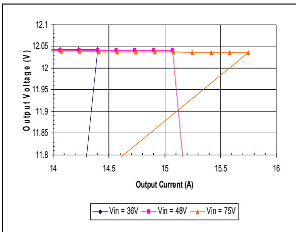
iQB48012A120V-000 Typical Output Current Limit Characteristics vs. Input Voltage at Ta=25 degrees.
