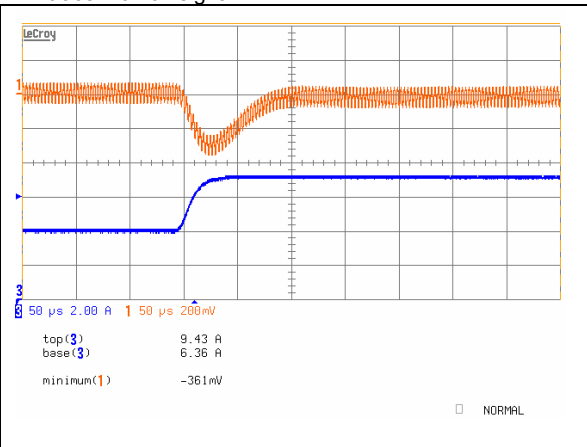
iQB48012A120V-000 Typical transient response. Output voltage response to load step from 50% to 75% of full load with output current slew rate of 0.1A/μs.
