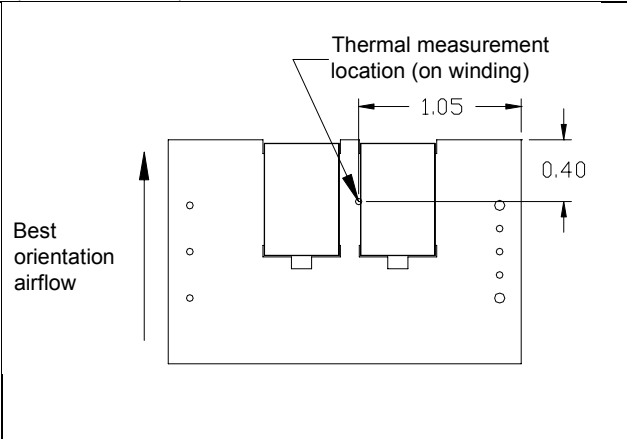
iQB48008A120V-000 thermal measurement location – top view
