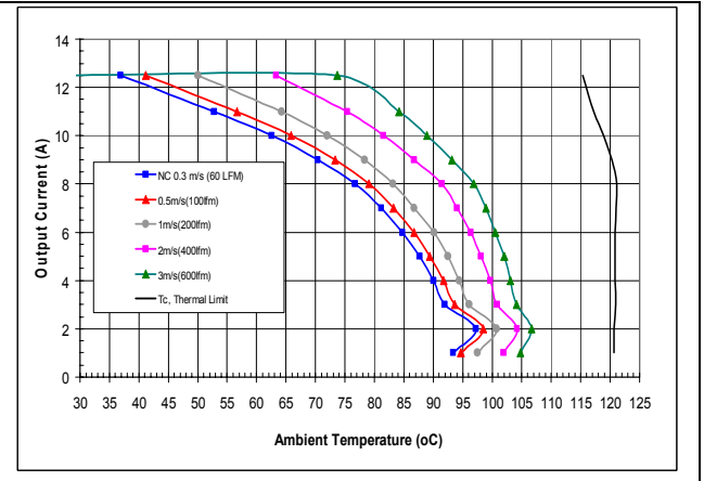
iQB48012A120V-000 maximum output current vs. ambient temperature at nominal input voltage for airflow rates natural convection (60lfm) to 600lfm with airflow from pin 1 to pin 3.
