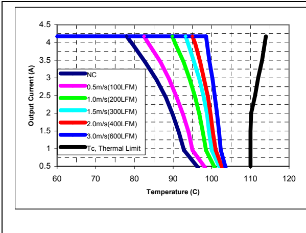
iQB48004A120V-000 maximum output current vs. ambient temperature at nominal input voltage for airflow rates natural convection (60lfm) to 600lfm with airflow from pin 3 to pin 1 (best orientation).
