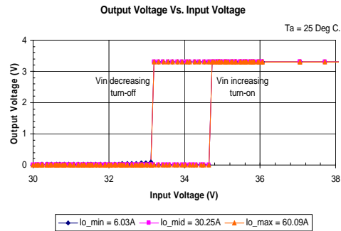
iHA48060A033V-000 Typical Output Voltage vs. Input Voltage Turn-on / Turn-off Characteristics – low voltage at Ta=25 degrees.
