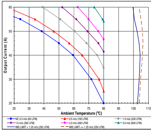
iHA48060A033V-000 maximum output current vs. ambient temperature at nominal input voltage for airflow rates natural convection 0.3 m/s (60lfm) to 3.0m/s (600lfm) with airflow from output to input.
