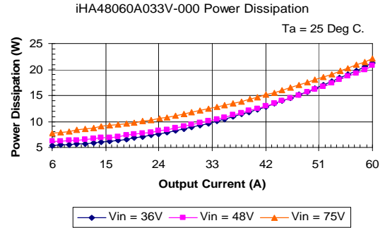
iHA48060A033V-000 Typical Power Dissipation vs. Output Current at Ta=25 degrees
