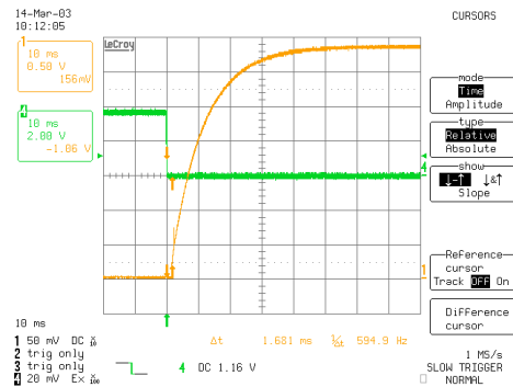
iHA48060A033V-000 Typical startup characteristic from on/off at full load. Upper trace - on/off signal, lower trace – output voltage
