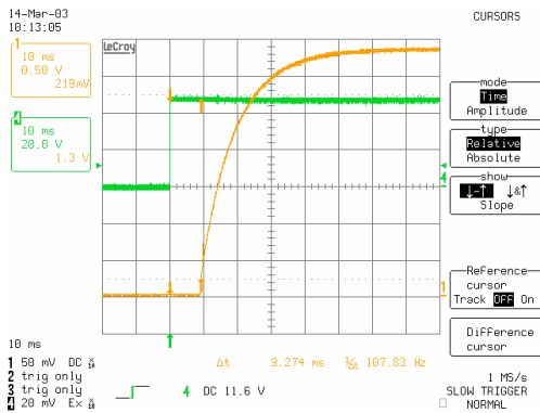
iHA48060A033V-000 Typical startup characteristic from input voltage application at full load. Upper trace - input voltage, lower trace – output voltage
