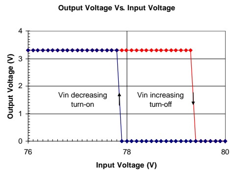
iHA48060A033V-000 Typical Output Voltage vs. Input Voltage Turn-on / Turn-off Characteristics – high voltage at Ta=25 degrees.
