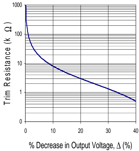
iHA48060A033V-000 Trim down curve for output voltage adjustment
