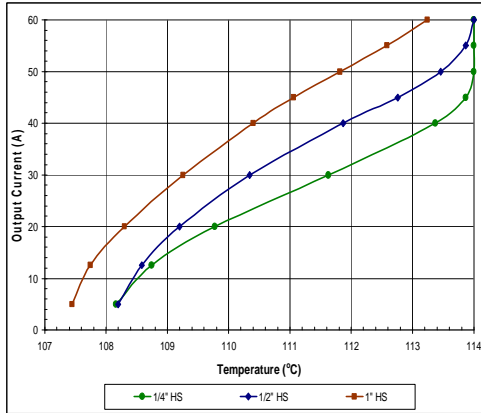
iHA48060A033V-000 with heatsink maximum Output Current vs. maximum allowable IMS Temperature at nominal input voltage with airflow from output to input.
