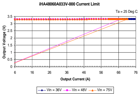
iHA48060A033V-000 Typical Output Current Limit Characteristics vs. Input Voltage at Ta=25 degrees.
