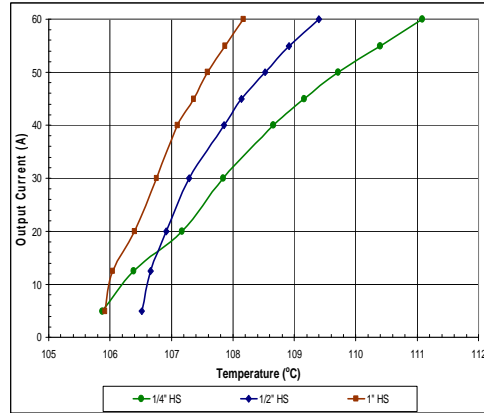
iHA48060A033V-000 with heatsink maximum Output Current vs. maximum allowable IMS Temperature at nominal input voltage with airflow from input to output.
