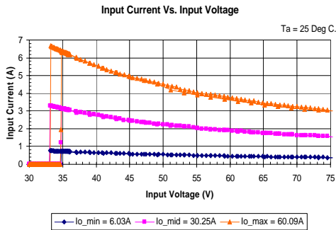
iHA48060A033V-000 Typical Input Current vs. Input Voltage Characteristics at Ta=25 degrees.
