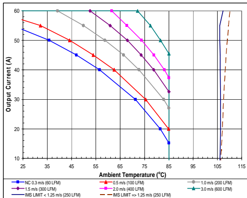
iHA48060A033V-000 maximum output current vs. ambient temperature at nominal input voltage for airflow rates natural convection 0.3 m/s (60lfm) to 3.0m/s (600lfm) with airflow from input to output.
