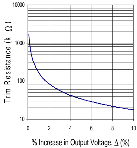
iHA48060A033V-000 Trim up curve for output voltage adjustment
