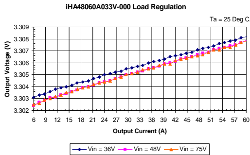
iHA48060A033V-000 Typical Output Voltage vs. Load Current at Ta = 25 degrees
