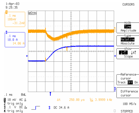
iHA48060A033V-000 Typical transient response. Load step from 50% to 75% of full load with 0.1A/uS. Lower trace – output current , upper trace – output voltage
