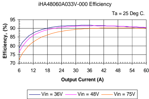
iHA48060A033V-000 Typical Efficiency vs. Output Current at Ta=25 degrees.
