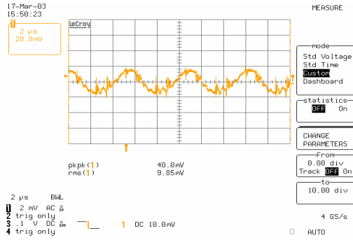
iHA48060A033V-000 Typical Output Ripple at nominal Input voltage and full load with external capacitors 47uF+1uF+0.1uF at Ta=25 degrees
