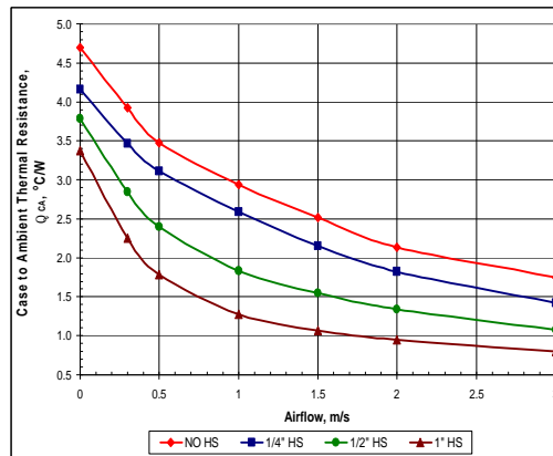
iHA48060A033V-000 Case to Ambient Thermal Resistance vs. Airflow rate
