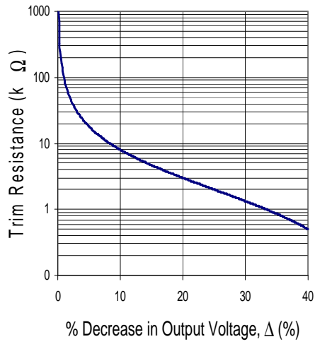
iHA48040A050V-001 Trim down curve for output voltage adjustment
