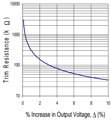
iHA48040A050V-001 Trim up curve for output voltage adjustment
