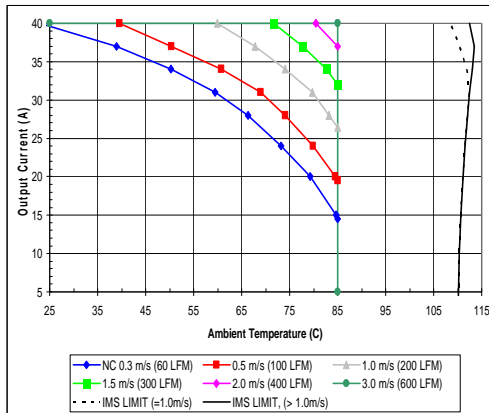
iHD48040A050V-001 maximum output current vs. ambient temperature at nominal input voltage for airflow rates natural convection 0.3 m/s (60lfm) to 3.0m/s (600lfm) with airflow from output to input.
