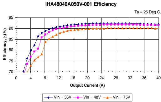
iHA48040A050V-001 Typical Efficiency vs. Output Current at Ta=25 degrees.
