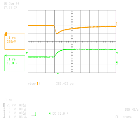
iHA48040A050V-001 Typical transient response. Load step from 50% to 75% of full load with 0.1A/uS. Lower trace - output current, upper trace - output voltage
