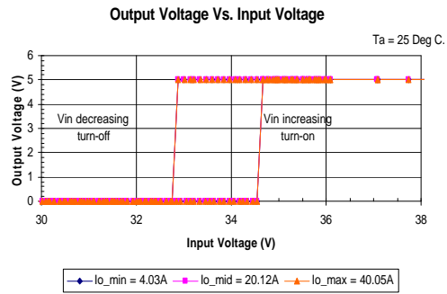
iHA48040A050V-001 Typical Output Voltage vs. Input Voltage Turn-on / Turn-off Characteristics – low voltage at Ta=25 degrees.
