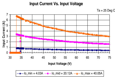
iHA48040A050V-001 Typical Input Current vs. Input Voltage Characteristics at Ta=25 degrees.
