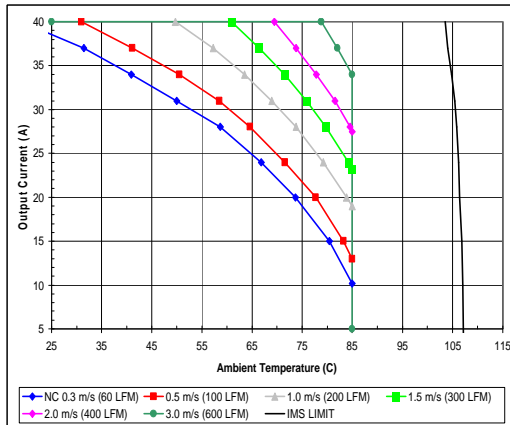
iHA48040A050V-001 maximum output current vs. ambient temperature at nominal input voltage for airflow rates natural convection 0.3 m/s (60lfm) to 3.0m/s (600lfm). Airflow from Vout (-) to Vout (+) with the module output side on the left
