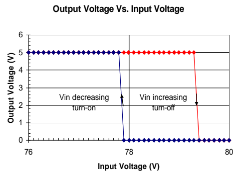
iHA48040A050V-001 Typical Output Voltage vs. Input Voltage Turn-on / Turn-off Characteristics – high voltage at Ta=25 degrees.
