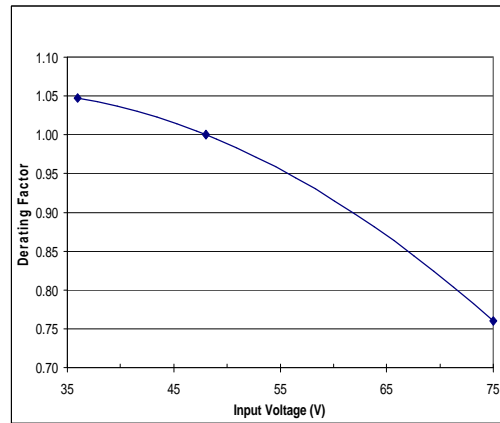
iHA48040A050V-001 Output Current Derating Factor vs. Input Voltage for 25°C < Ta < 85°C and Io > 10A
