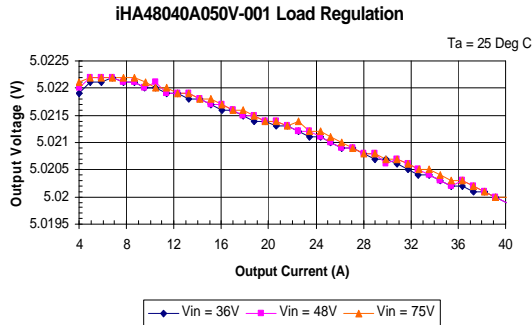
iHA48040A050V-001 Typical Output Voltage vs. Load Current at Ta = 25 degrees
