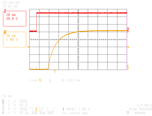
iHA48040A050V-001 Typical startup characteristic from input voltage application at full load. Upper trace - input voltage, lower trace - output voltage
