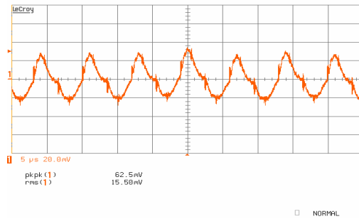
iHA48040A050V-001 Typical Output Ripple at nominal Input voltage and full load with external capacitors 10uF+1uF+0.1uF at Ta=25 degrees
