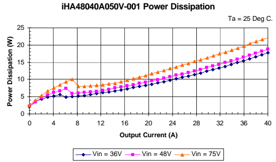
iHA48040A050V-001 Typical Power Dissipation vs. Output current at Ta=25 degrees
