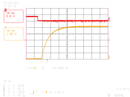
iHA48040A050V-001 Typical startup characteristic from on/off at full load. Upper trace - on/off signal, lower trace - output voltage
