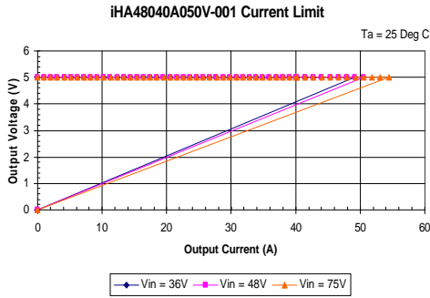
iHA48040A050V-001 Typical Output Current Limit Characteristics vs. Input Voltage at Ta=25 degrees.
