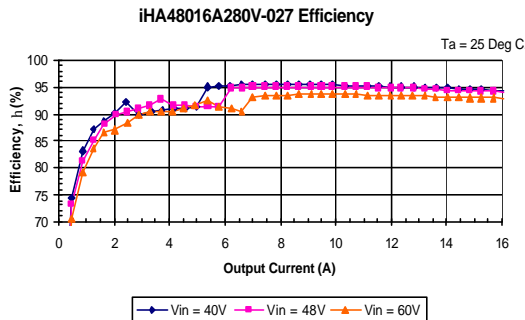
iHA48016A280V-027 Typical Efficiency vs. Output Current at Ta=25 degrees.
