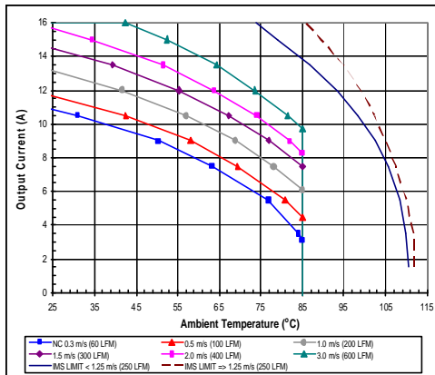
iHA48016A280V-027 maximum output current vs. ambient temperature at nominal input voltage for airflow rates natural convection 0.3 m/s (60lfm) to 3.0m/s (600lfm) with airflow from output to input.
