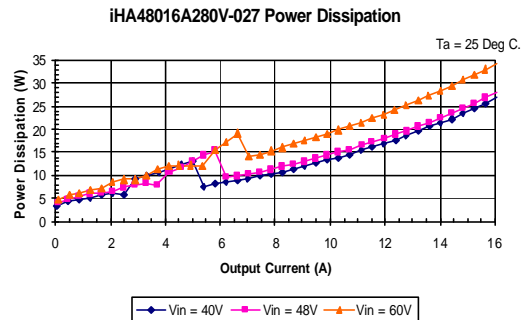
iHA48016A280V-027 Typical Power Dissipation vs. Output current at Ta=25 degrees
