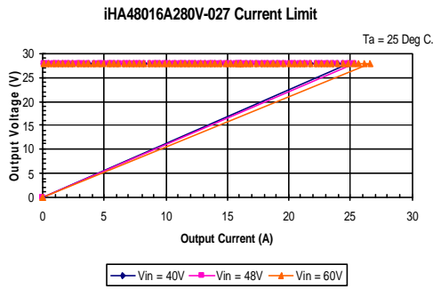
iHA48016A280V-027 Typical Output Current Limit Characteristics vs. Input Voltage at Ta=25 degrees.
