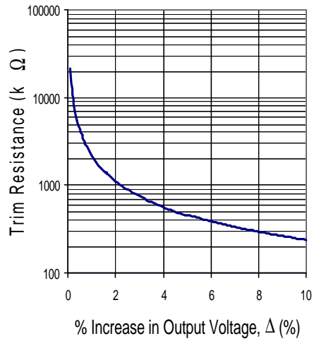
iHA48016A280V-027 Trim up curve for output voltage adjustment
