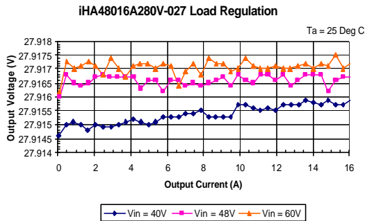
iHA48016A280V-027 Typical Output Voltage vs. Load Current at Ta = 25 degrees
