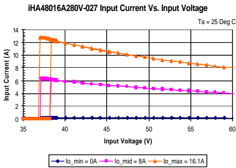
iHA48016A280V-027 Typical Input Current vs. Input Voltage Characteristics at Ta=25 degrees.
