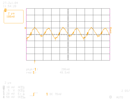
iHA48016A280V-027 Typical Output Ripple at nominal Input voltage and full load with external capacitors 200uF Al +10uF+1uF+0.1uF ceramic at Ta=25 degrees
