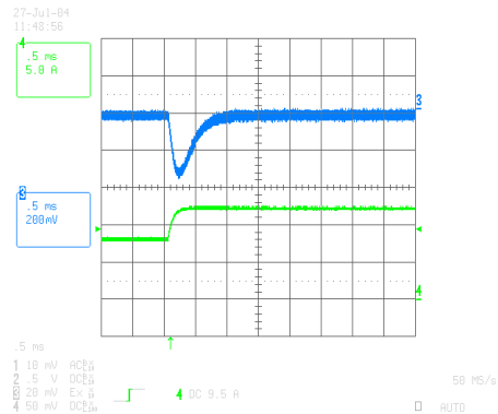
iHA48016A280V-027 Typical transient response. Load step from 50% to 75% of full load with 0.1A/uS. Lower trace – output current, upper trace – output voltage
