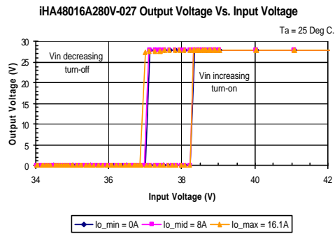
iHA48016A280V-027 Typical Output Voltage vs. Input Voltage Turn-on / Turn-off Characteristics – low voltage at Ta=25 degrees.
