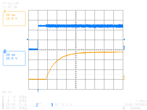
iHA48016A280V-027 Typical startup characteristic from input voltage application at full load. Upper trace - input voltage, lower trace – output voltage
