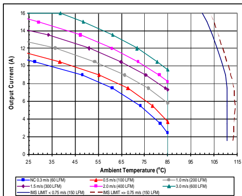
iHA48016A280V-027 maximum output current vs. ambient temperature at nominal input voltage for airflow rates natural convection 0.3 m/s (60lfm) to 3.0m/s (600lfm). Airflow from Vin (+) to Vin (-) with the module output side on the left.
