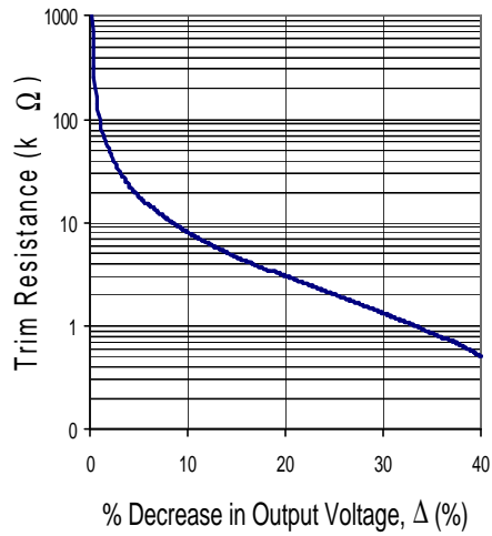
iHA48016A280V-027 Trim down curve for output voltage adjustment
