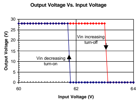
iHA48016A280V-027 Typical Output Voltage vs. Input Voltage Turn-on / Turn-off Characteristics – high voltage at Ta=25 degrees.
