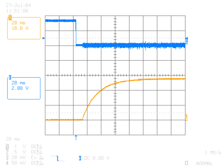
iHA48016A280V-027 Typical startup characteristic from on/off at full load. Upper trace - on/off signal, lower trace – output voltage
