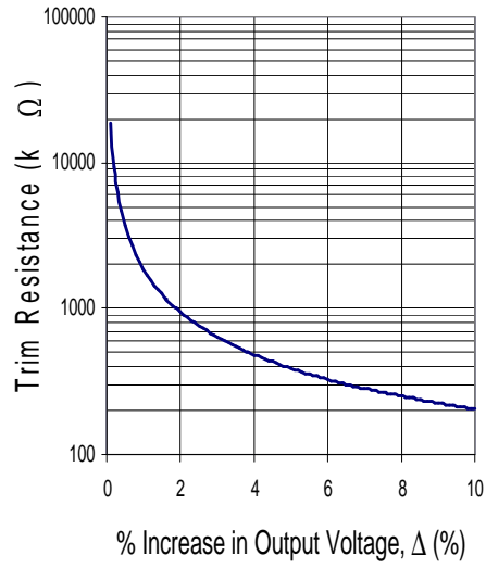
iHA48013A240V-001 Trim up curve for output voltage adjustment
