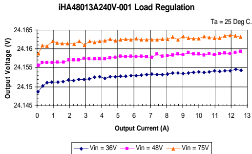
iHA48013A240V-001 Typical Output Voltage vs. Load Current at Ta = 25 degrees
