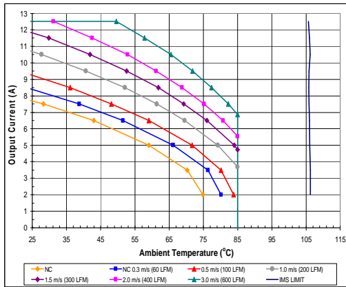
iHA48013A240V-001 maximum output current vs. ambient temperature at nominal input voltage for airflow rates natural convection 0.3 m/s (60lfm) to 3.0m/s (600lfm) with airflow from input to output.
