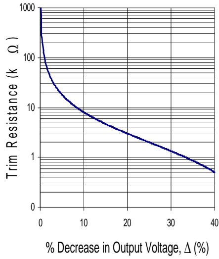
iHA48013A240V-001 Trim down curve for output voltage adjustment
