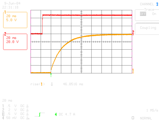
iHA48013A240V-001 Typical startup characteristic from input voltage application at full load. Upper trace - input voltage, lower trace - output voltage
