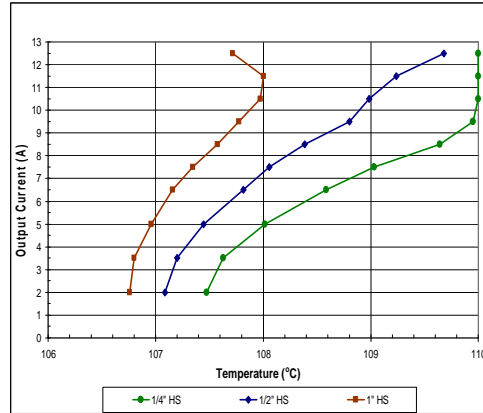
iHA48013A240V-001 with heatsink maximum Output Current vs. maximum allowable IMS Temperature at nominal input voltage with airflow from input to output.
