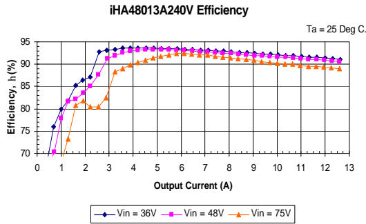
iHA48013A240V-001 Typical Efficiency vs. Output Current at Ta=25 degrees.
