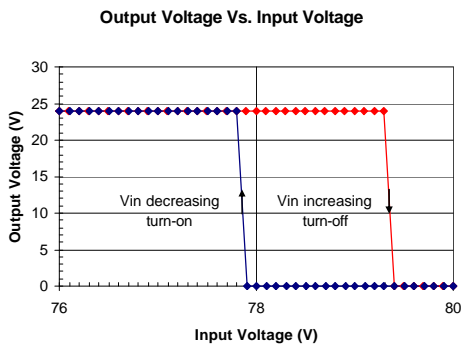
iHA48013A240V-001 Typical Output Voltage vs. Input Voltage Turn-on / Turn-off Characteristics – high voltage at Ta=25 degrees.
