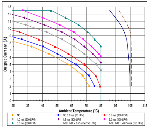
iHA48013A240V-001 maximum output current vs. ambient temperature at nominal input voltage for airflow rates natural convection 0.3 m/s (60lfm) to 3.0m/s (600lfm). Airflow from Vin(-) to Vin(+) with the module output side on the left.
