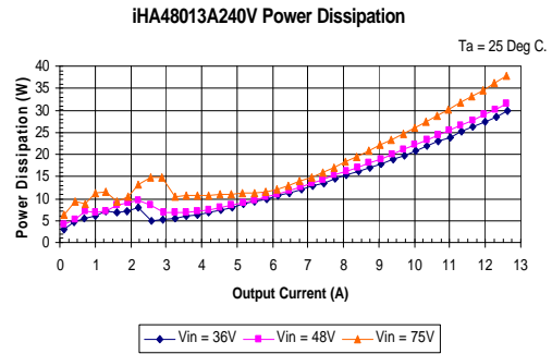
iHA48013A240V-001 Typical Power Dissipation vs. Output current at Ta=25 degrees
