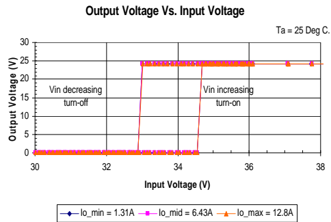
iHA48013A240V-001 Typical Output Voltage vs. Input Voltage Turn-on / Turn-off Characteristics – low voltage at Ta=25 degrees.
