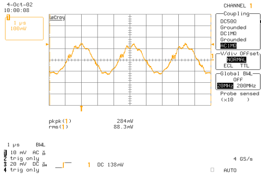
iHA48013A240V-001 Typical Output Ripple at nominal Input voltage and full load with external capacitors 200uF Al +10uF+1uF+0.1uF ceramic at Ta=25 degrees
