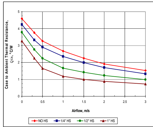
iHA48013A240V-001 Case to Ambient Thermal Resistance vs. Airflow rate
