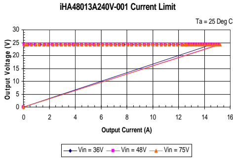
iHA48013A240V-001 Typical Output Current Limit Characteristics vs. Input Voltage at Ta=25 degrees.
