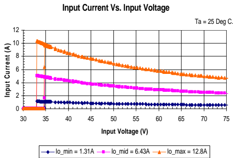
iHA48013A240V-001 Typical Input Current vs. Input Voltage Characteristics at Ta=25 degrees.
