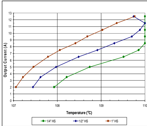
iHA48013A240V-001 with heatsink maximum Output Current vs. maximum allowable IMS Temperature at nominal input voltage. Airflow from Vin(-) to Vin(+) with the module output side on the left.
