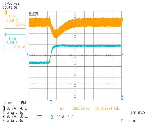
iHA48013A240V-001 Typical transient response. Load step from 50% to 75% of full load with 0.1A/uS. Lower trace - output current, upper trace - output voltage
