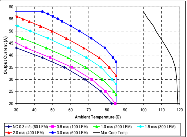
Maximum output current vs. ambient temperature at nominal input voltage with no base plate for airflow rates natural convection (0.3m/s) to 3.0m/s with airflow from pin 1 to pin 4.
