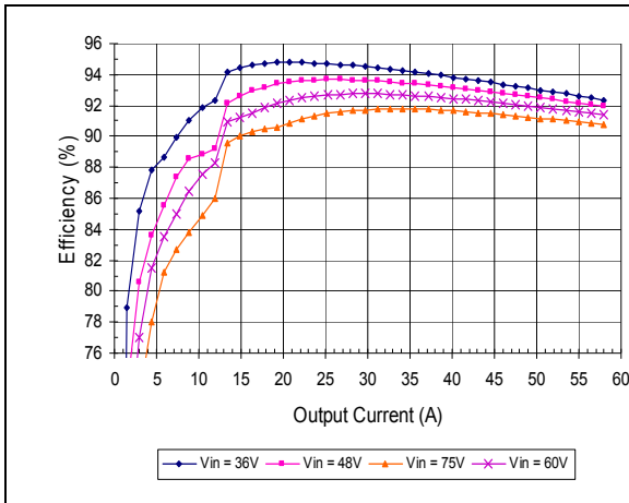
Typical Efficiency vs. Vin and Load (tested in socket, no base-plate)
