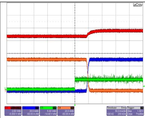
Start-up with back-biased at nominal input and 50A load. Ch.1: Vo Ch.2: lo2 (starting) Ch. 3: ON/OFF Ch. 4: lo1 (running)
