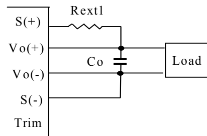
Figure Trim up Connection
