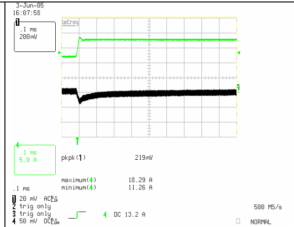
Typical Dynamic Load Response. Load step from 50% to 75% of full load, di/dt = 0.1A/μs. (Note: Vin=48V) Ch. 1: Output Voltage, Ch. 4: Load Current
