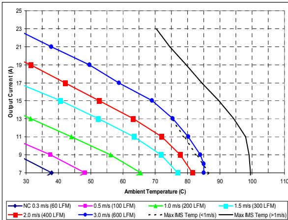
Maximum output current vs. ambient temperature at nominal input voltage (no heat sink) for airflow rates natural convection (0.3 m/s (60lfm) to 3.0m/s (600lfm)) with airflow from Vout(+) pins to Vout(-) pins.
