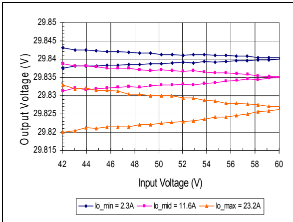
Output Voltage vs. Input Voltage (Line Regulation) at Ta=25 °C.
