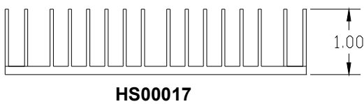
Transverse Heatsinks
