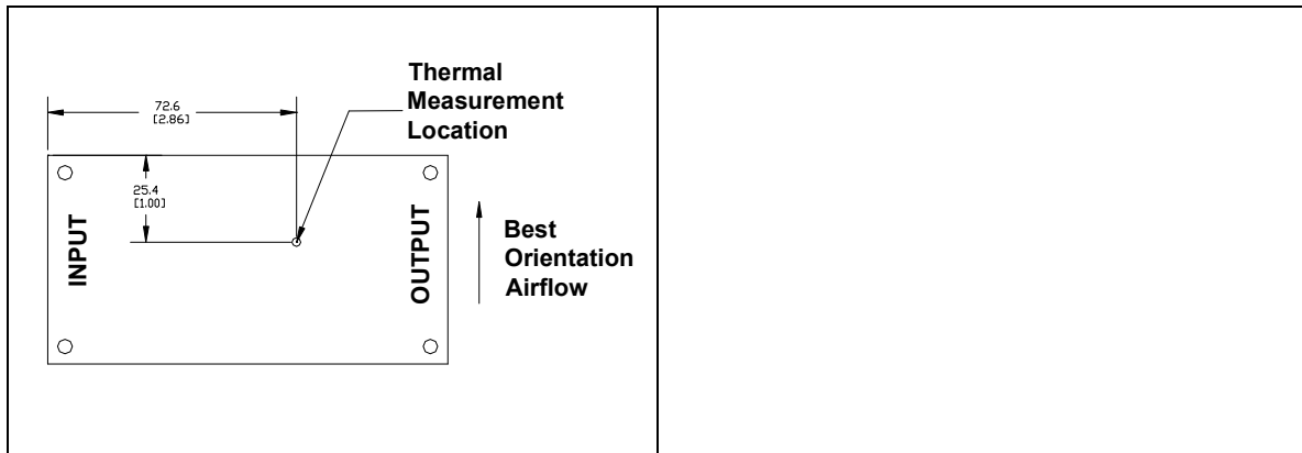
Thermal measurement location – top view
