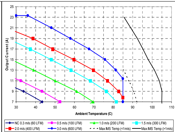
Maximum output current vs. ambient temperature at nominal input voltage (no heat sink) for airflow rates natural convection (0.3m/s (60lfm) to 3.0m/s (600lfm)) with airflow from Vout(-) pins to Vout(+) pins.
