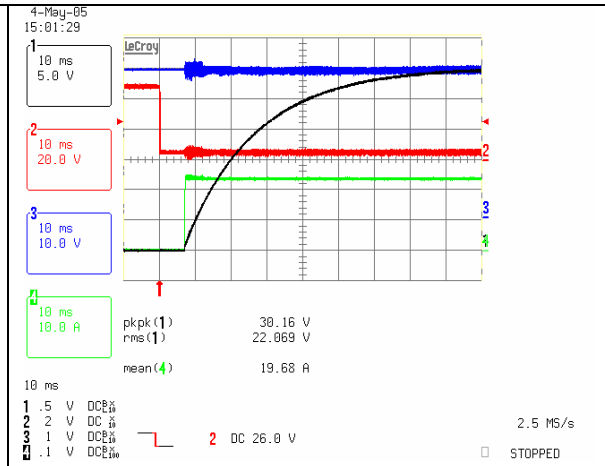
Start-up from ON/OFF switch at nominal Vin and full load. Ch.1: Vout Ch. 2: ON/OFF Ch.3: Vin, Ch.4: Io
