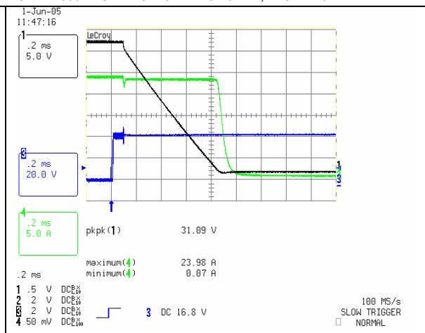
Typical Output Voltage Fall Characteristics at Vin=48V, Io=23A Ch. 1: Vo Ch. 3: ON/OFF Ch. 4: Io
