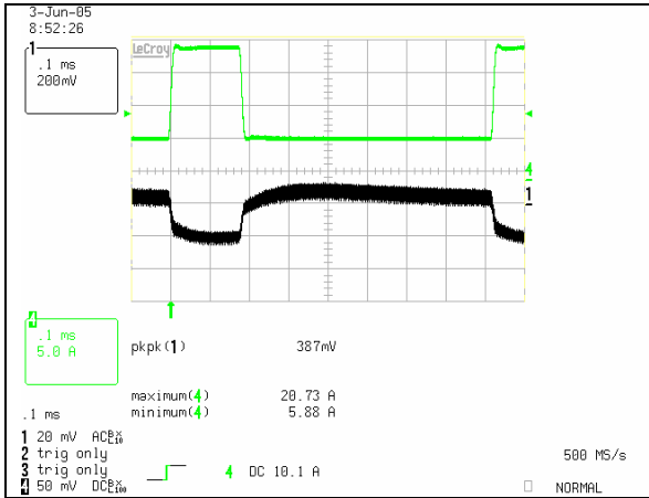
Dynamic Load Transient. Load step from 25% to 86% of full load with 1.2kHz, di/dt = 1A/μs (Cext=2680μF) Ch. 1: Vo Ch. 4: Io
