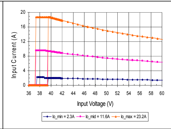
Input Start-up Current vs. Line and Load Current at Ta=25 °C
