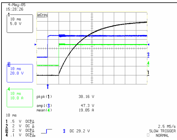
Start-up from input voltage application and full load. Ch.1: Vout Ch.3: Vin Ch.4: Load Current
