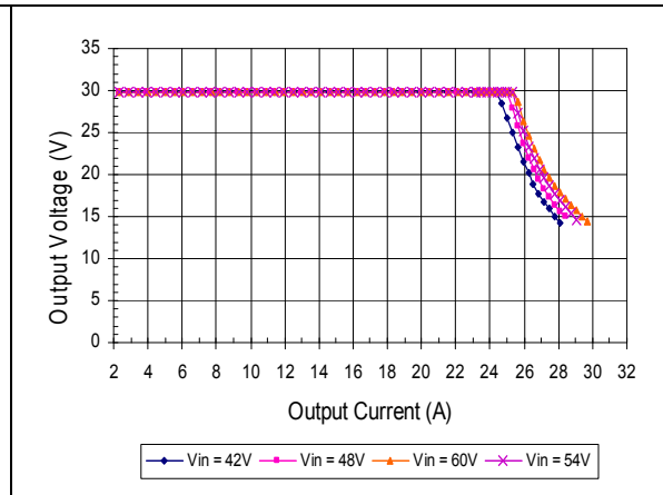
Typical Current Limit vs. Input Voltage at Ta=25 °C
