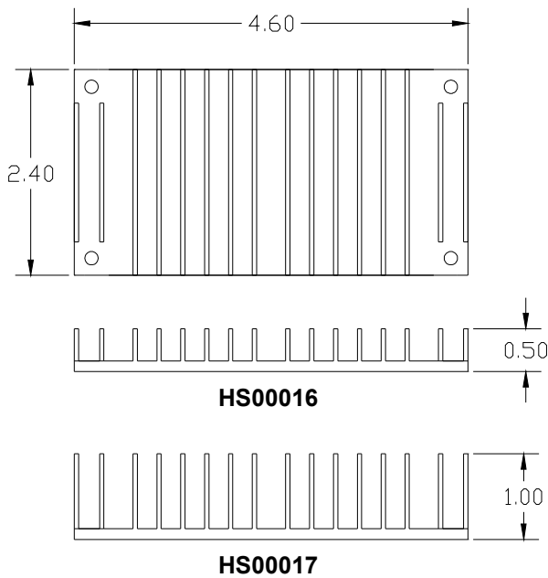
Transverse Heatsinks
