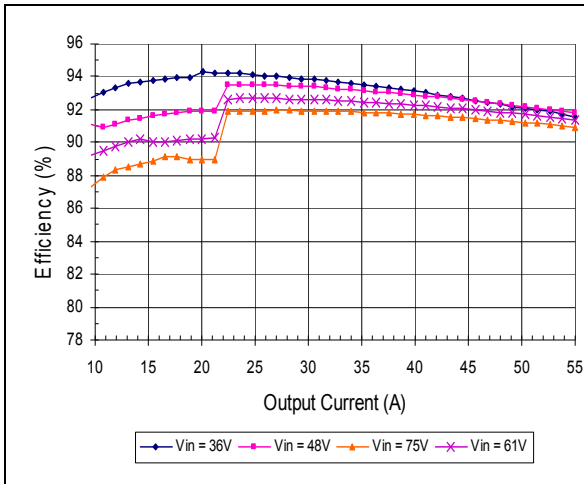
Typical Efficiency vs. Input Voltage and Load (use test socket)
