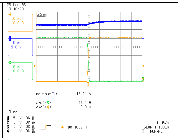
Start-up with back-biased voltage at nominal input and 50A load. Turn-on from Vin application while the load share line disconnected Ch.1: Vo Ch.3: Io2 (running) Ch. 4: Io1 (starting unit)
