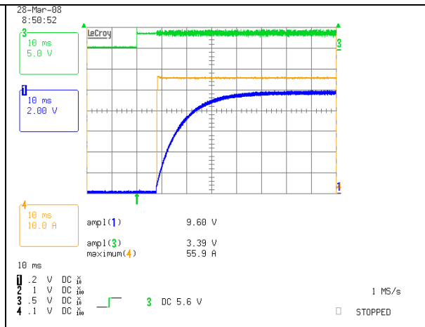
Start-up Characteristics from ON/OFF switch at nominal input and full load. Ch.1: Vo Ch.3: ON/OFF Ch.4: Io
