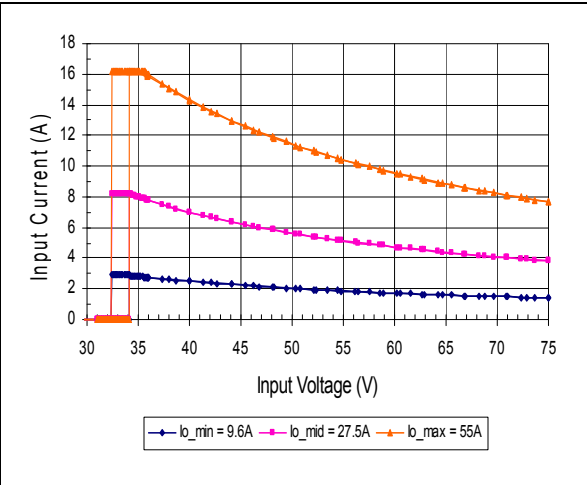
Typical Input Start-up Current vs. Load Current
