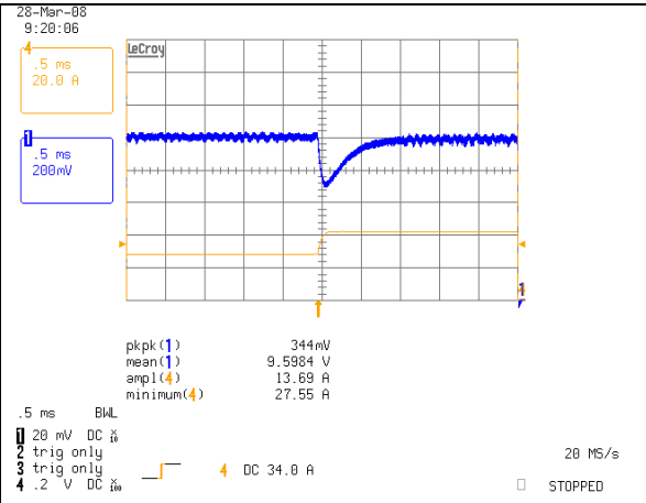
Typical Dynamic Load Response. Load step from 50% to 75% of full load, di/dt= 0.1A/μS. Vin=48V Ch. 1: Vo Ch. 4: Io
