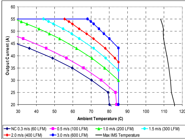
Maximum output current vs. ambient temperature at nominal input voltage for airflow rates natural convection (0.3 m/s) to 3.0 m/s with airflow from Vout(+) pins to Vout(-) pins.
