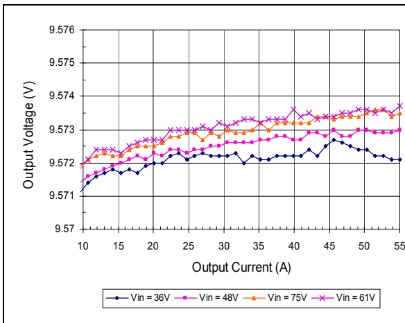
Typical Output Voltage vs. Load Current (use test socket)
