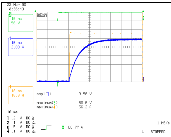
Start-up Characteristics from input voltage application at full load. Ch.1: Vo Ch.3: Vin Ch.4: Io
