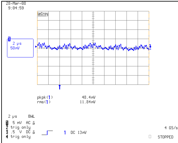
Typical Output Ripple at Nominal Input Voltage and Full Load Ch. 1: Vo
