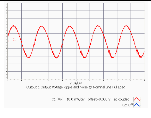
iEF48013A050V-000 Typical Output Ripple at nominal input voltage and full load at Ta=25 degrees
