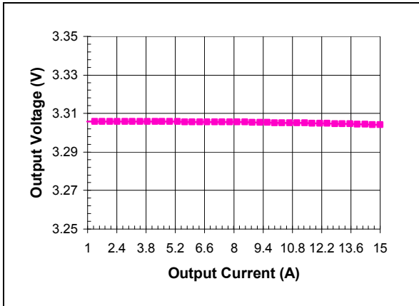
iEF48015A033V-000 Typical Output Voltage vs. Load Current at Ta = 25 degrees
