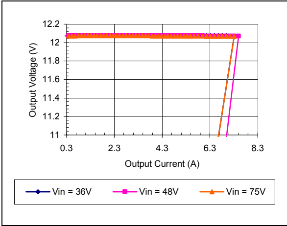
iEF48006A120V-000 Typical Output Current Limit Characteristics vs. Input Voltage at Ta=25 degrees.
