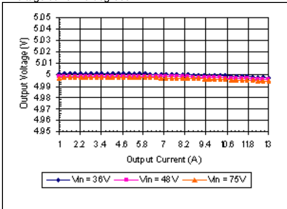
iEF48013A050V-000 Typical Output Voltage vs. Load Current at Ta = 25 degrees
