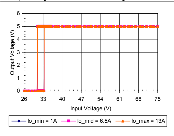
iEF48013A050V-000 Typical Output Voltage vs. Input Voltage Characteristics
