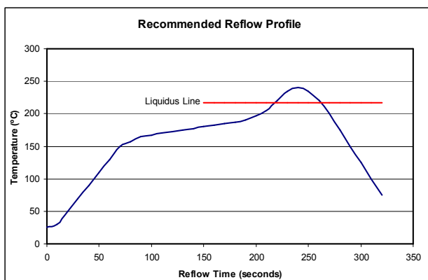
iEF Power Module suggested reflow-soldering profile
