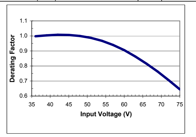
iEF48006A120V-000 typical output current derating versus line voltage
