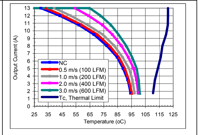
iEF48013A050V-000 maximum output current vs. ambient temperature at nominal input voltage for airflow rates natural convection (60lfm) to 600lfm with airflow from pin 6 to pin 2.
