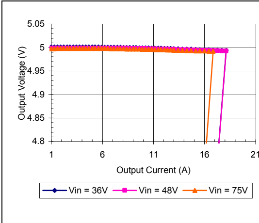
iEF48013A050V-000 Typical Output Current Limit Characteristics vs. Input Voltage at Ta=25 degrees.
