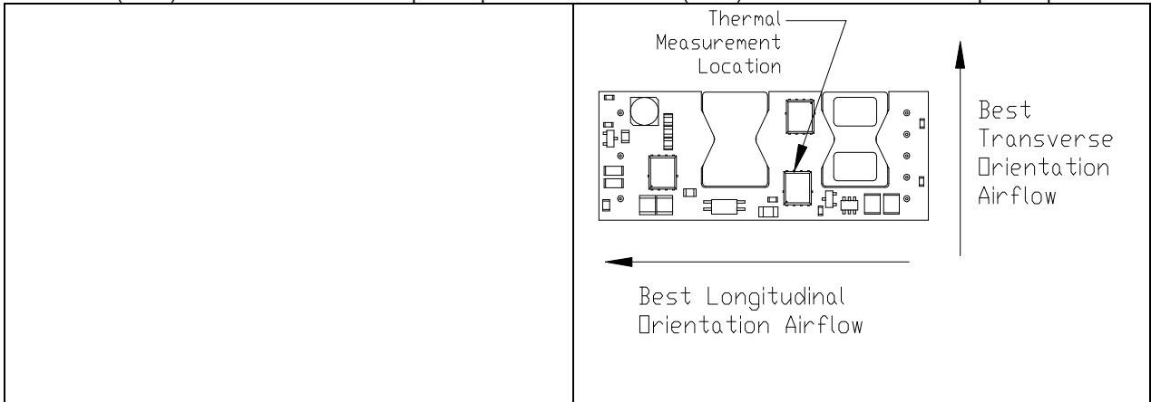
iEF48015A033V-000 thermal measurement location – top view
