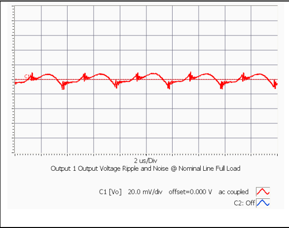
iEF48006A120V-000 Typical Output Ripple at nominal input voltage and full load at Ta=25 degrees
