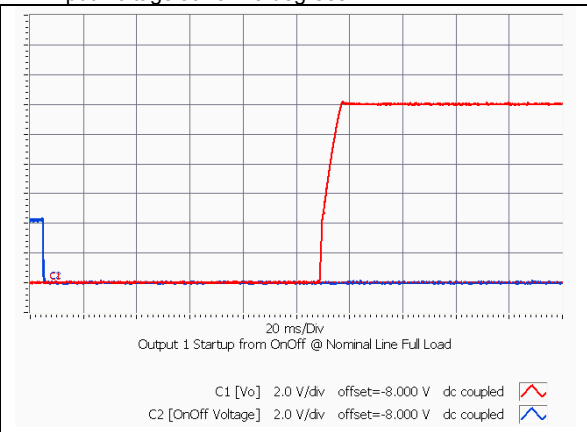
iEF48006A120V-001 Typical startup characteristic from on/off at full load. Ch 2 - on/off signal, Ch 1 – output voltage
