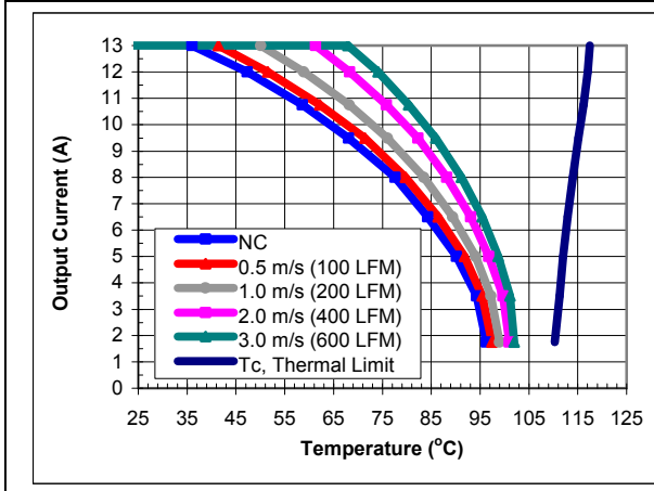
iEF48013A050V-000 maximum output current vs. ambient temperature at nominal input voltage for airflow rates natural convection (60lfm) to 600lfm with airflow from pin 3 to pin 1.
