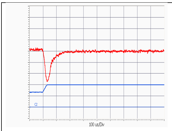
iEF48013A050V-000 Typical Output voltage response, 50mV/div to load step from 50% to 75% of full load with output current slew rate of 0.1A/uS.
