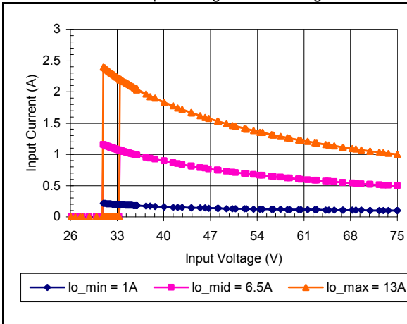
iEF48013A050V-000 Typical Input Current vs. Input Voltage Characteristics
