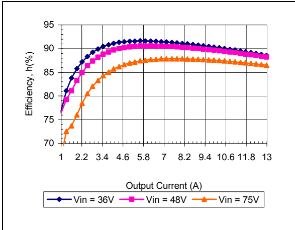
iEF48013A050V-000 Typical Efficiency vs. Input Voltage at Ta=25 degrees.
