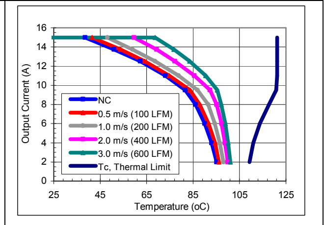
iEF48015A033V-000 maximum output current vs. ambient temperature at nominal input voltage for airflow rates natural convection (60lfm) to 600lfm with airflow from pin 6 to pin 2.
