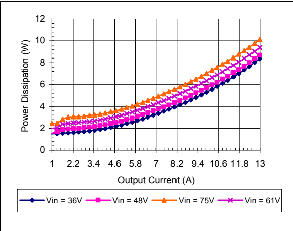
iEF48013A050V-000 Typical Power Dissipation vs. Input Voltage at Ta=25 degrees
