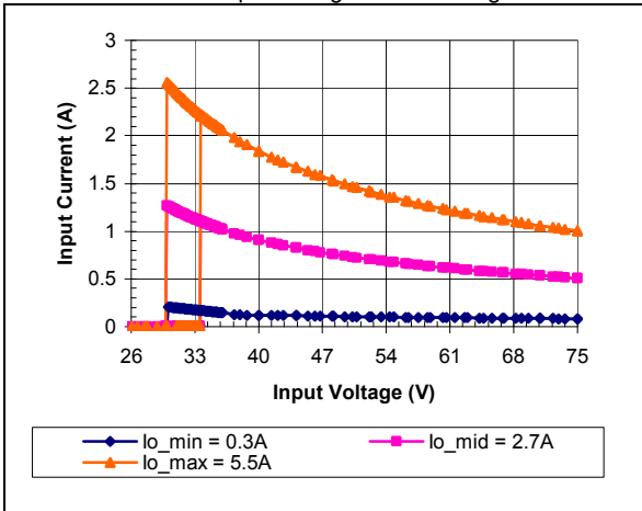
iEF48006A120V-000 Typical Input Current vs. Input Voltage Characteristics
