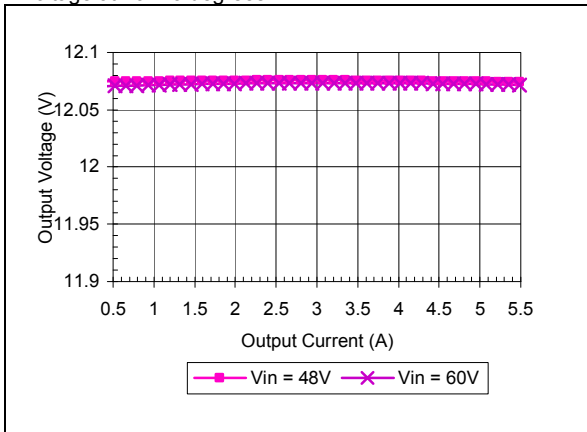
iEF48006A120V-000 Typical Output Voltage vs. Load Current at Ta = 25 degrees
