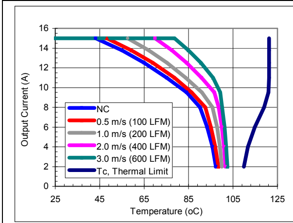
iEF48015A033V-000 maximum output current vs. ambient temperature at nominal input voltage for airflow rates natural convection (60lfm) to 600lfm with airflow from pin 3 to pin 1.
