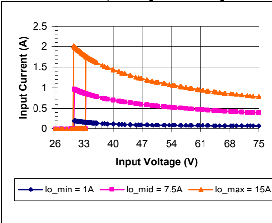
iEF48015A033V-000 Typical Input Current vs. Input Voltage Characteristics
