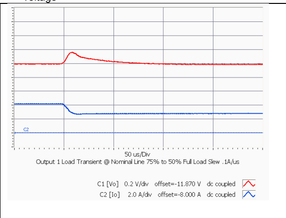
iEF48006A120V-000 Typical Output voltage response to load step from 75% to 50% of full load with output current slew rate of 0.1A/uS.
