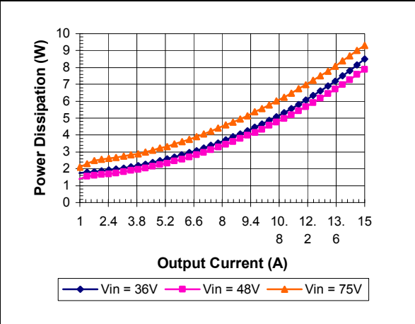
iEF48015A033V-000 Typical Power Dissipation vs. Input Voltage at Ta=25 degrees
