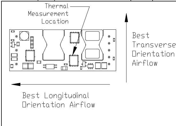
iEF48006A120V-000 thermal measurement location – top view
