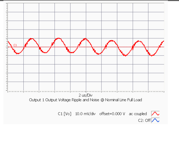
iEF48015A033V-000 Typical Output Ripple at nominal input voltage and full load at Ta=25 degrees.
