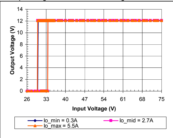
iEF48006A120V-000 Typical Output Voltage vs. Input Voltage Characteristics
