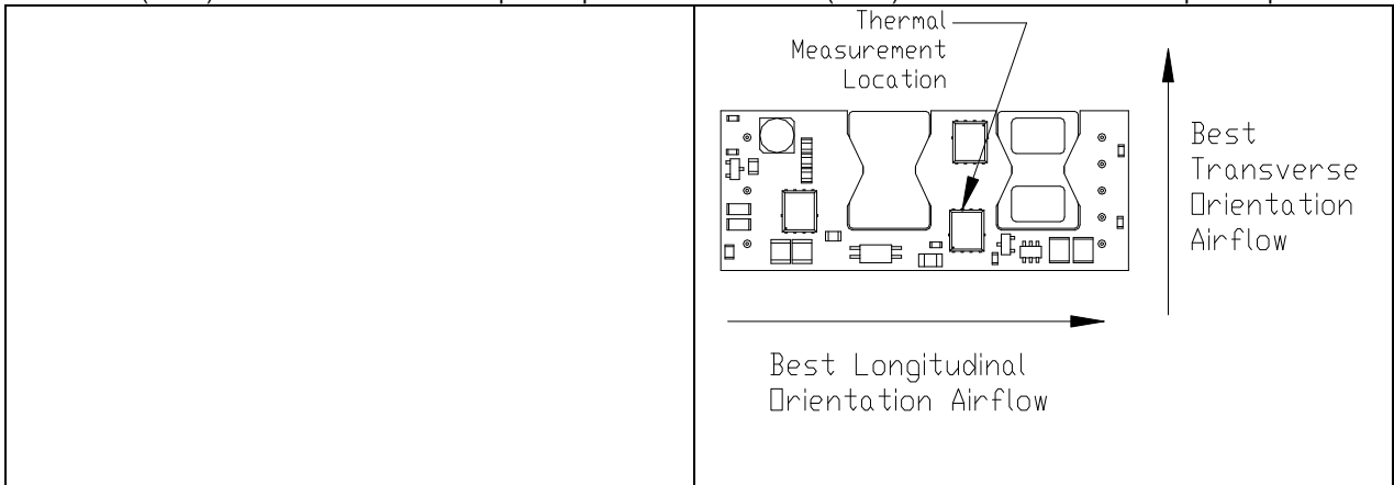
iEF48013A050V-000 thermal measurement location – top view
