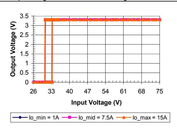
iEF48015A033V-000 Typical Output Voltage vs. Input Voltage Characteristics
