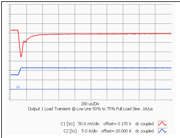
iEF48015A033V-000 Typical output voltage response to load step from 50% to 75% of full load with output current slew rate of 0.1A/uS and 200uF load.
