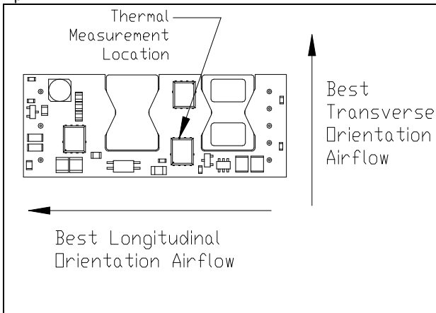
iEE4W004A120V-000 thermal measurement location – top view
