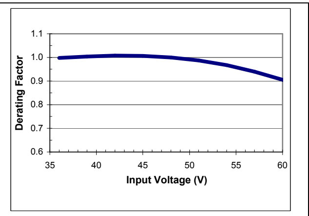
iEE4W004A120V-000 typical output current derating versus line voltage
