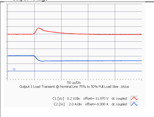
iEE4W004A120V-000 Typical Output voltage response to load step from 75% to 50% of full load with output current slew rate of 0.1A/uS.
