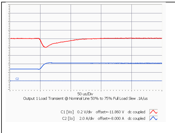
iEE4W004A120V-000 Typical Output voltage response to load step from 50% to 75% of full load with output current slew rate of 0.1A/uS.
