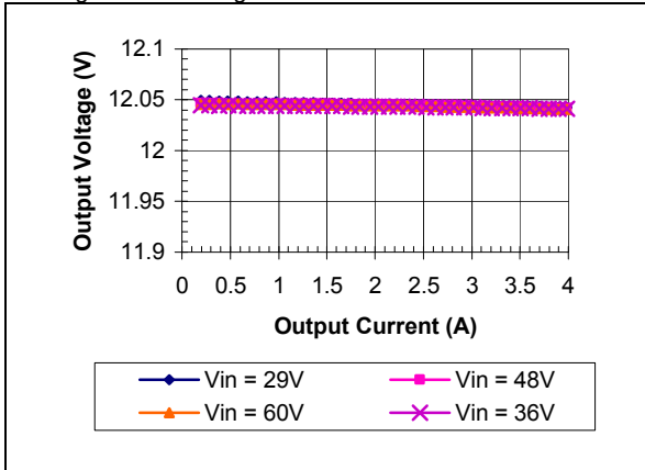
iEE4W004A120V-000 Typical Output Voltage vs. Load Current at Ta = 25 degrees
