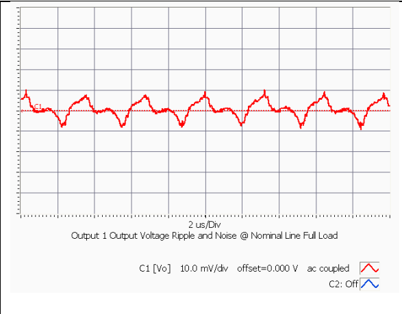
iEE4W004A120V-000 Typical Output Ripple at nominal input voltage and full load at Ta=25 degrees
