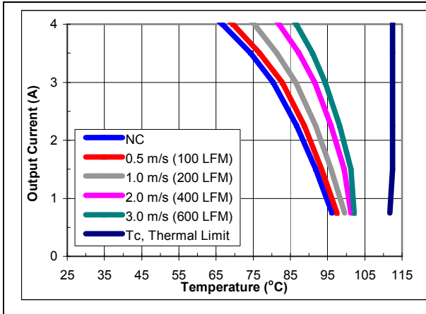
iEE4W004A120V-000 estimated maximum output current vs. ambient temperature at nominal input voltage for airflow rates natural convection (60lfm) to 600lfm with airflow from pin 3 to pin 1.
