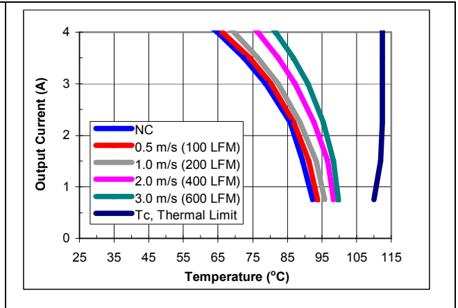
iEE4W004A120V-000 estimated maximum output current vs. ambient temperature at nominal input voltage for airflow rates natural convection (60lfm) to 600lfm with airflow from pin 6 to pin 2.
