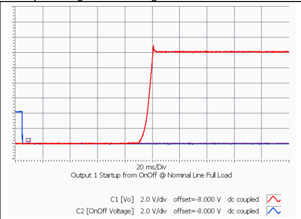
iEE4W004A120V-001 Typical startup characteristic from on/off at full load. Ch 2 - on/off signal, Ch 1 - output voltage
