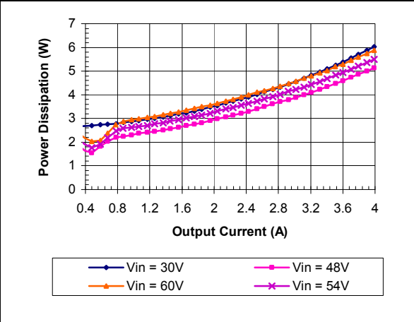
iEE4W004A120V-000 Typical Power Dissipation vs. Input Voltage at Ta=25 degrees
