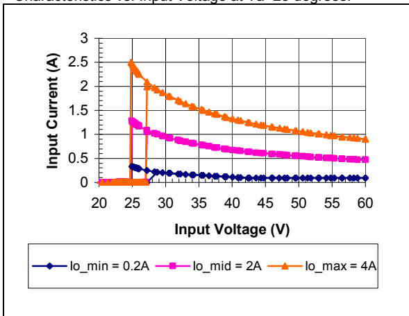
iEE4W004A120V-000 Typical Input Current vs. Input Voltage Characteristics
