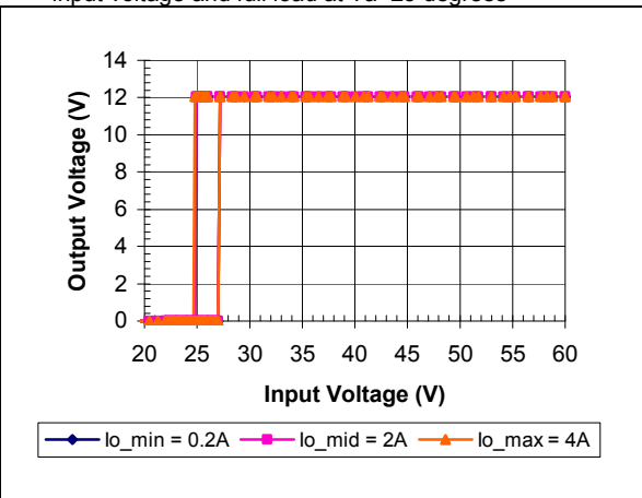
iEE4W004A120V-000 Typical Output Voltage vs. Input Voltage Characteristics
