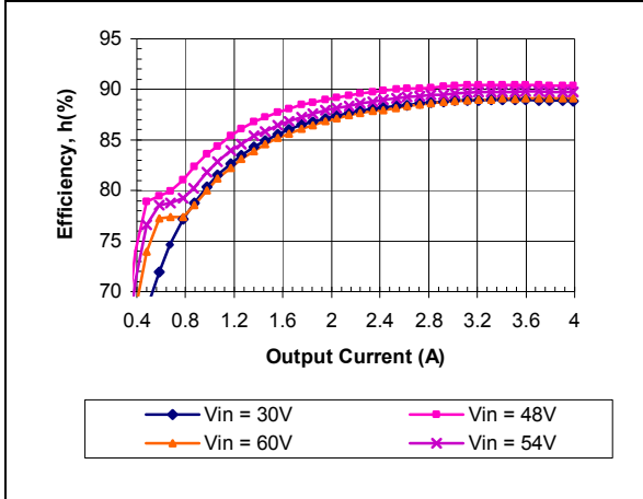
iEE4W004A120V-000 Typical Efficiency vs. Input Voltage at Ta=25 degrees.
