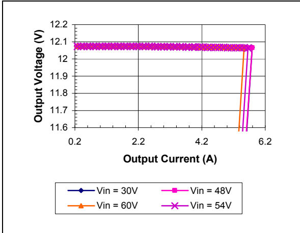
iEE4W004A120V-000 Typical Output Current Limit Characteristics vs. Input Voltage at Ta=25 degrees.
