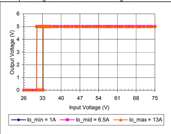
iEE48013A050V-000 Typical Output Voltage vs. Input Voltage Characteristics
