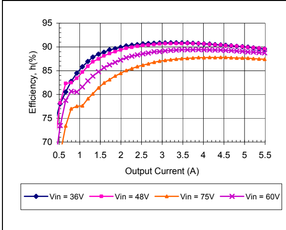
iEE48006A120V-000 Typical Efficiency vs. Input Voltage at Ta=25 degrees.
