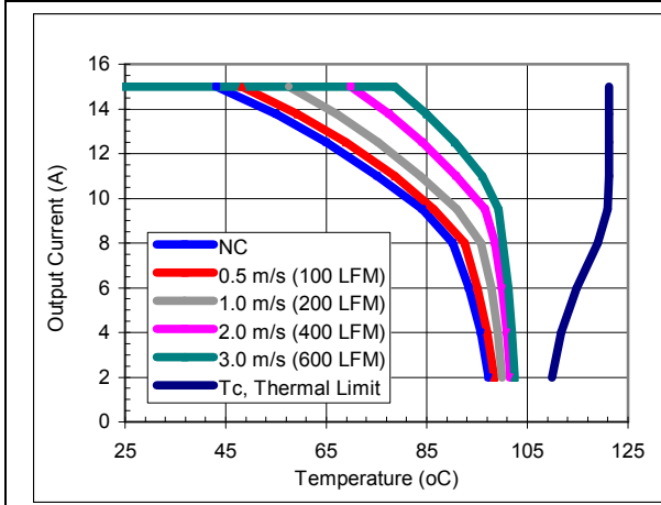
iEE48015A033V-000 maximum output current vs. ambient temperature at nominal input voltage for airflow rates natural convection (60lfm) to 600lfm with airflow from pin 3 to pin 1.
