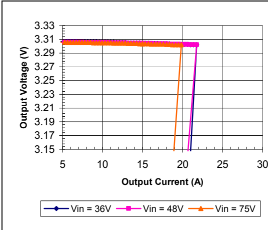
iEE48015A033V-000 Typical Output Current Limit Characteristics vs. Input Voltage at Ta=25 degrees.
