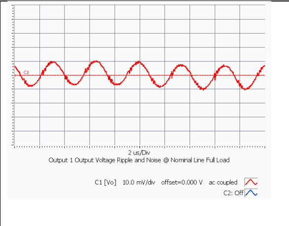
iEE48015A033V-000 Typical Output Ripple at nominal input voltage and full load at Ta=25 degrees.
