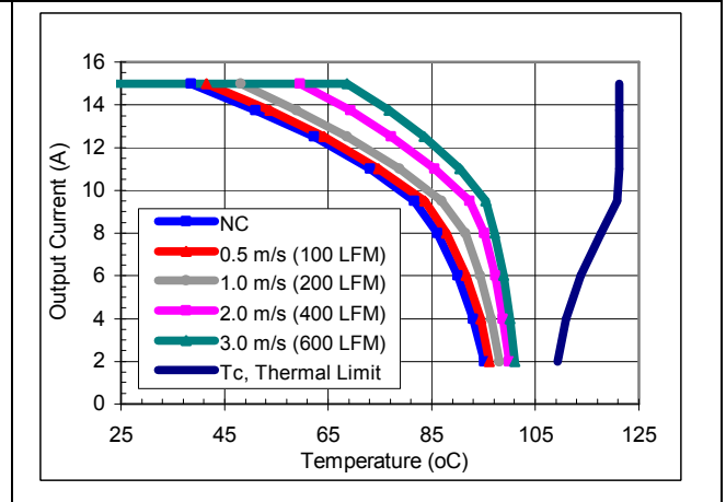
iEE48015A033V-000 maximum output current vs. ambient temperature at nominal input voltage for airflow rates natural convection (60lfm) to 600lfm with airflow from pin 6 to pin 2.
