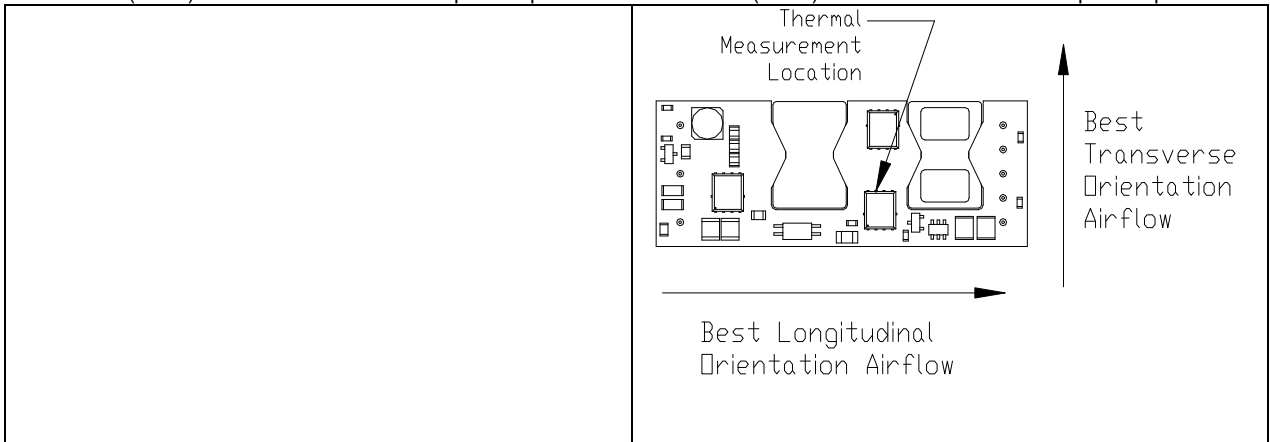
iEE48013A050V-000 thermal measurement location – top view
