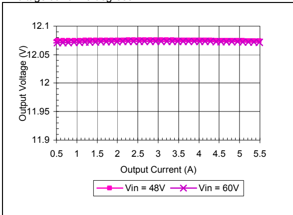
iEE48006A120V-000 Typical Output Voltage vs. Load Current at Ta = 25 degrees
