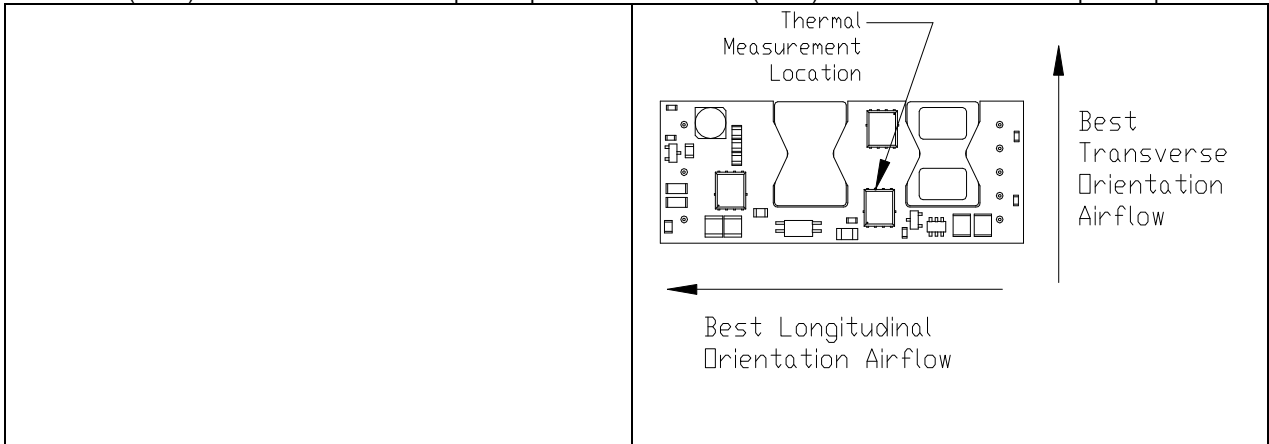
iEE48015A033V-000 thermal measurement location – top view
