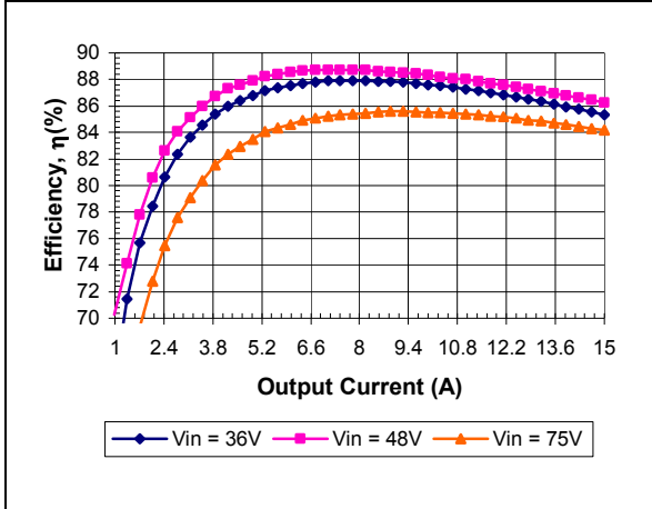
iEE48015A033V-000 Typical Efficiency vs. Input Voltage at Ta=25 degrees.
