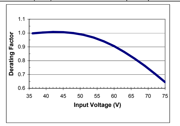
iEE48006A120V-000 typical output current derating versus line voltage
