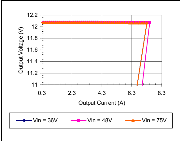
iEE48006A120V-000 Typical Output Current Limit Characteristics vs. Input Voltage at Ta=25 degrees.
