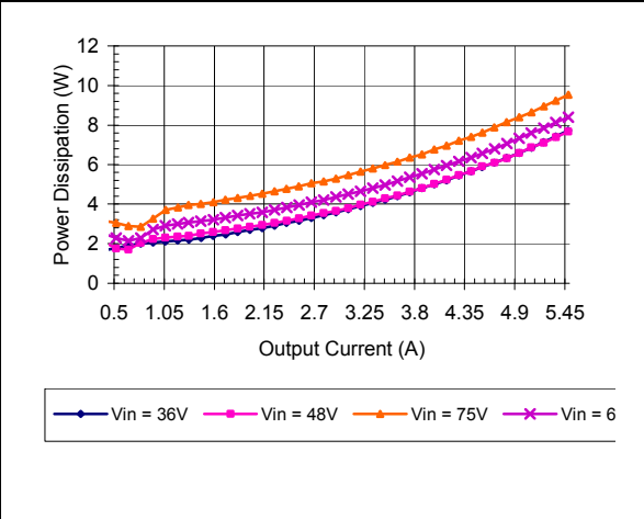
iEE48006A120V-000 Typical Power Dissipation vs. Input Voltage at Ta=25 degrees
