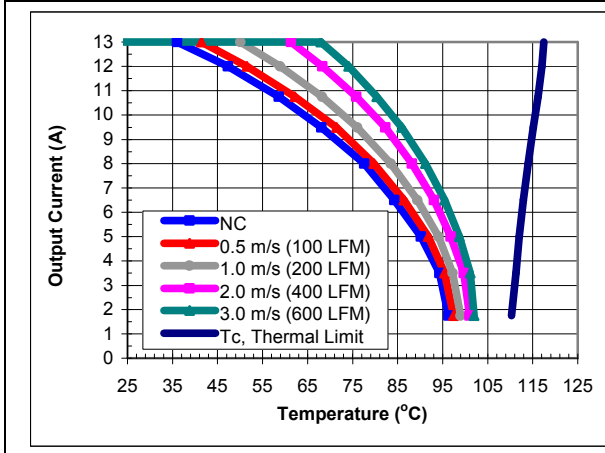
iEE48013A050V-000 maximum output current vs. ambient temperature at nominal input voltage for airflow rates natural convection (60lfm) to 600lfm with airflow from pin 3 to pin 1.
