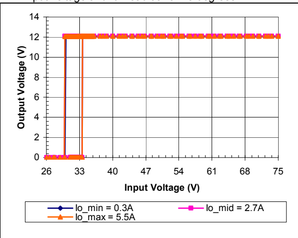
iEE48006A120V-000 Typical Output Voltage vs. Input Voltage Characteristics
