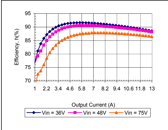
iEE48013A050V-000 Typical Efficiency vs. Input Voltage at Ta=25 degrees.
