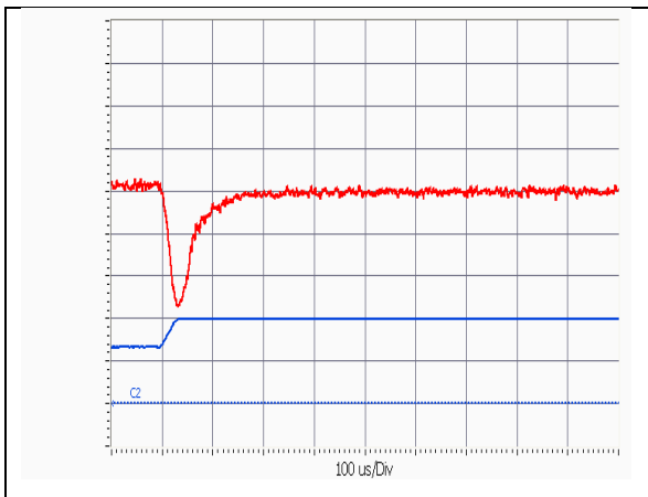
iEE48013A050V-000 Typical Output voltage response, 50mV/div to load step from 50% to 75% of full load with output current slew rate of 0.1A/uS.
