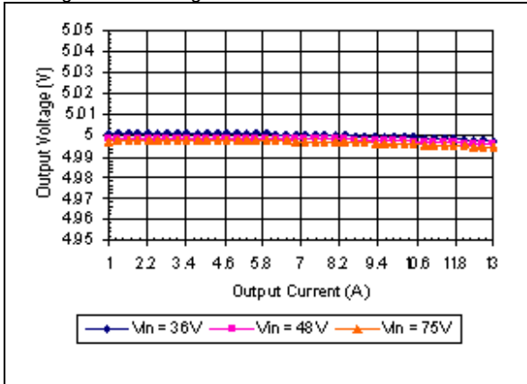
iEE48013A050V-000 Typical Output Voltage vs. Load Current at Ta = 25 degrees
