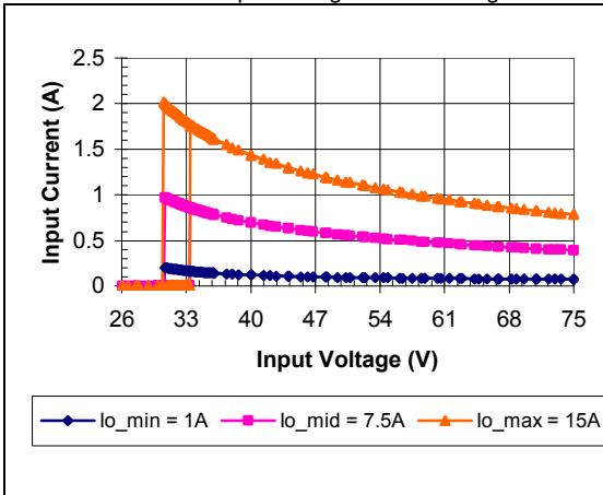
iEE48015A033V-000 Typical Input Current vs. Input Voltage Characteristics
