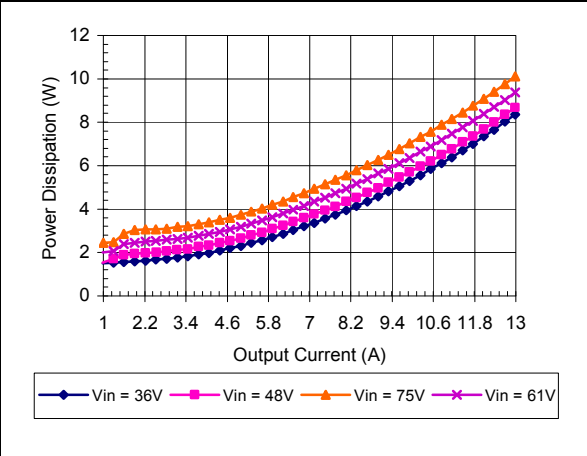
iEE48013A050V-000 Typical Power Dissipation vs. Input Voltage at Ta=25 degrees
