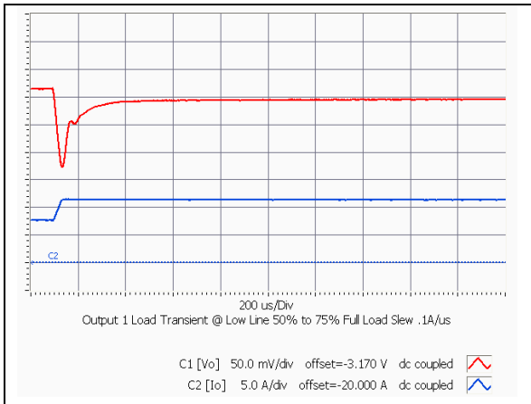
iEE48015A033V-000 Typical output voltage response to load step from 50% to 75% of full load with output current slew rate of 0.1A/uS and 200uF load.
