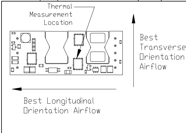
iEE48006A120V-000 thermal measurement location – top view
