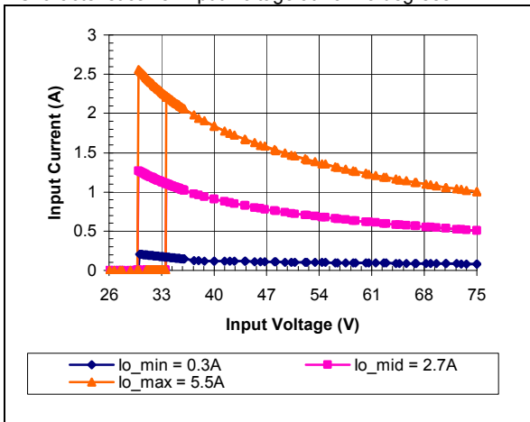
iEE48006A120V-000 Typical Input Current vs. Input Voltage Characteristics
