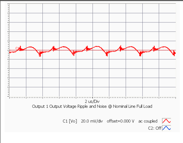
iEE48006A120V-000 Typical Output Ripple at nominal input voltage and full load at Ta=25 degrees
