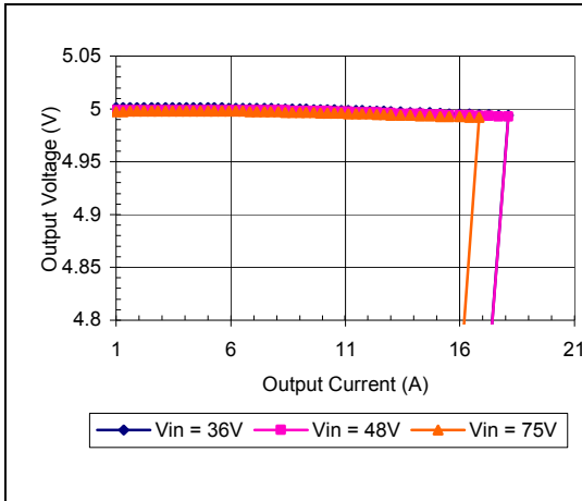
iEE48013A050V-000 Typical Output Current Limit Characteristics vs. Input Voltage at Ta=25 degrees.
