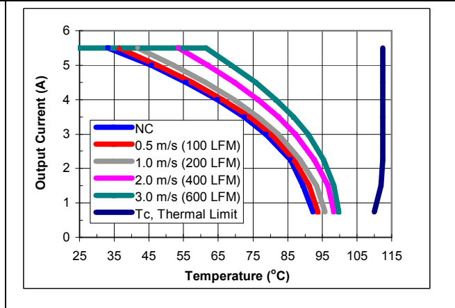
iEE48006A120V-000 maximum output current vs. ambient temperature at nominal input voltage for airflow rates natural convection (60lfm) to 600lfm with airflow from pin 6 to pin 2.
