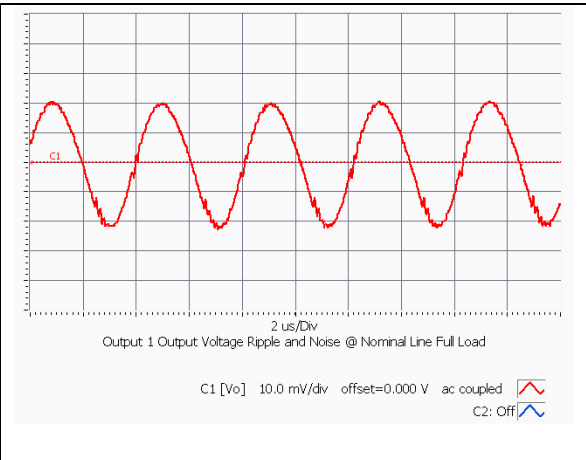
iEE48013A050V-000 Typical Output Ripple at nominal input voltage and full load at Ta=25 degrees
