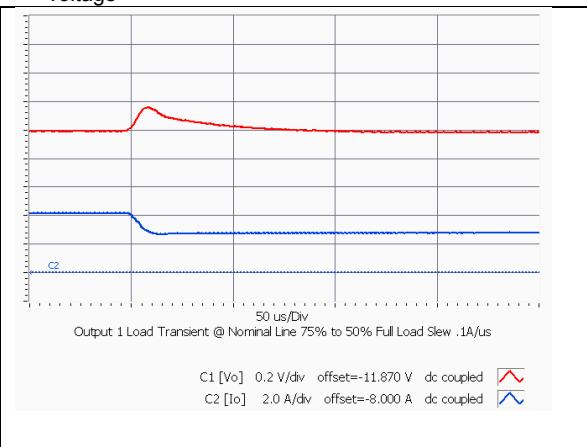
iEE48006A120V-000 Typical Output voltage response to load step from 75% to 50% of full load with output current slew rate of 0.1A/uS.
