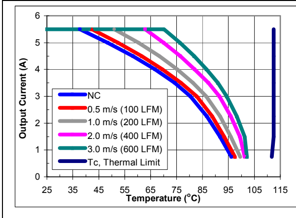
iEE48006A120V-000 maximum output current vs. ambient temperature at nominal input voltage for airflow rates natural convection (60lfm) to 600lfm with airflow from pin 3 to pin 1.
