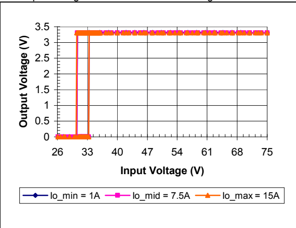
iEE48015A033V-000 Typical Output Voltage vs. Input Voltage Characteristics
