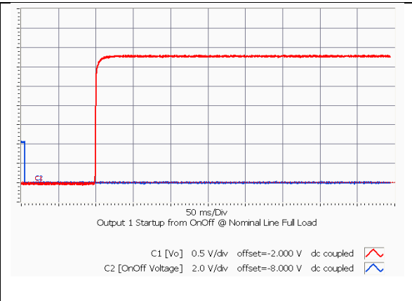
iEE48015A033V-001 Typical startup characteristic from on/off at full load. Ch2 - on/off signal, Ch 1 – output voltage
