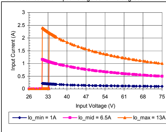
iEE48013A050V-000 Typical Input Current vs. Input Voltage Characteristics
