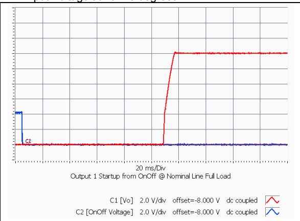
iEE48006A120V-001 Typical startup characteristic from on/off at full load. Ch 2 - on/off signal, Ch 1 – output voltage
