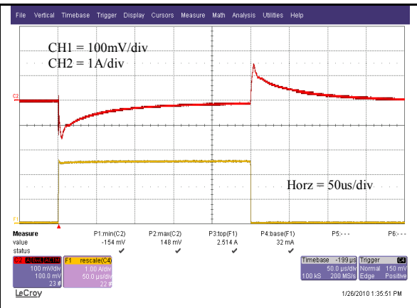
V_o=3.3V Typical output voltage transient response to load step from 0% to 50% of full load with output current slew rate of 10A/uS. (Cext = 2x22uF ceramic capacitor)
