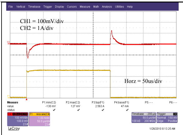
V_o=1.8V Typical output voltage transient response to load step from 25% to 75% of full load with output current slew rate of 10A/uS. (Cext = 2x22uF ceramic capacitor)
