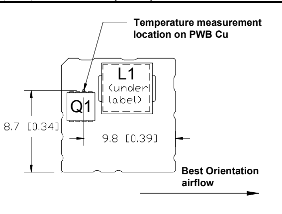
iCF12005A007V thermal measurement location – top view
