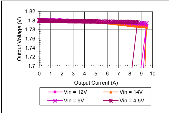
Vo=1.8V Typical Current Limit Characteristics
