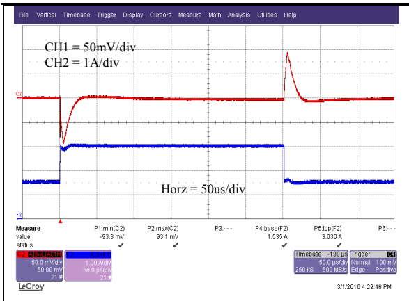
V_o=1.8V Typical output voltage transient response to load step from 50% to 100% of full load with output current slew rate of 10A/uS. (Cext = 2x22uF ceramic capacitor)
