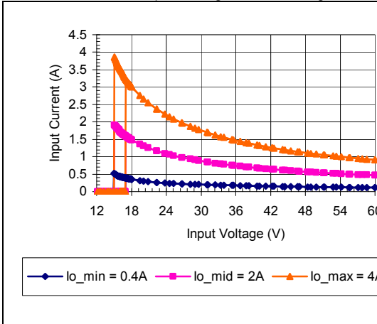
iEA4W004A120V-000 Typical Input Current vs. Input Voltage Characteristics
