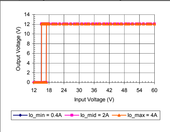
iEA4W004A120V-000 Typical Output Voltage vs. Input Voltage Characteristics
