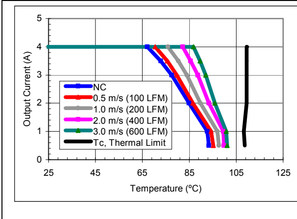
iEA4W004A120V-000 estimated maximum output current vs. ambient temperature at 48V input for airflow rates natural convection (60lfm) to 600lfm with airflow from pin 3 to pin 1.
