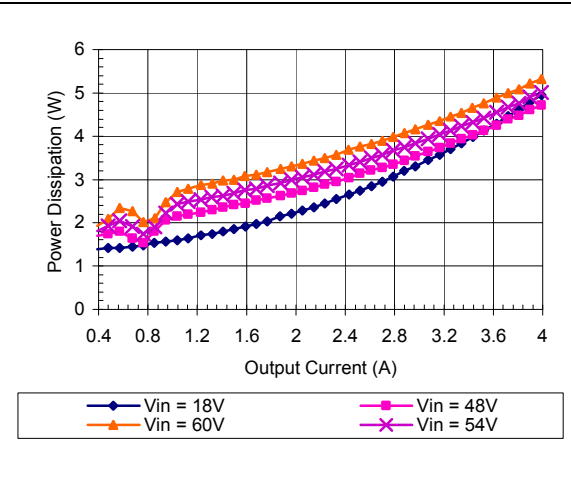
iEA4W004A120V-000 Typical Power Dissipation vs. Input Voltage at Ta=25 degrees
