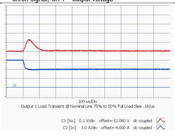
iEA4W004A120V-000 Typical Output voltage response to load step from 75% to 50% of full load with output current slew rate of 0.1A/uS and Cout = Co,min.
