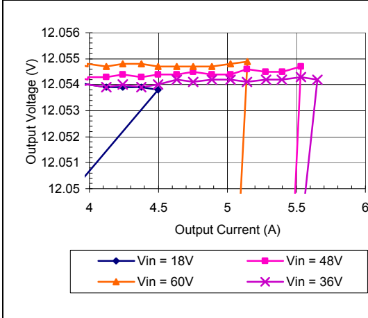
iEA4W004A120V-000 Typical Output Current Limit Characteristics vs. Input Voltage at Ta=25 degrees.
