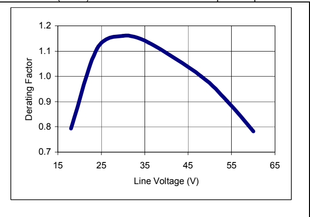
iEA4W004A120V-000 typical output current derating versus line voltage
