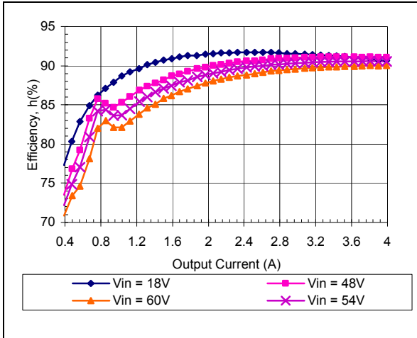
iEA4W004A120V-000 Typical Efficiency vs. Input Voltage at Ta=25 degrees.
