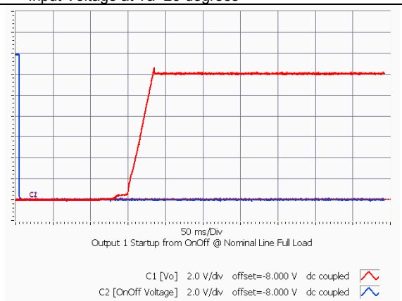
iEA4W004A120V-001 Typical startup characteristic from on/off at full load and Cout = Cout,min. Ch 2 - on/off signal, Ch 1 – output voltage
