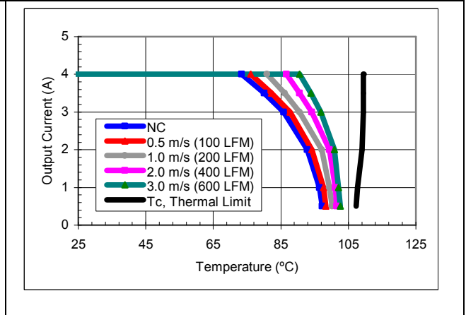
iEA4W004A120V-000 estimated maximum output current vs. ambient temperature at 24V input for airflow rates natural convection (60lfm) to 600lfm with airflow from pin 3 to pin 1.
