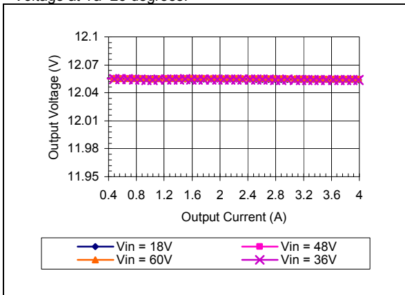
iEA4W004A120V-000 Typical Output Voltage vs. Load Current at Ta = 25 degrees
