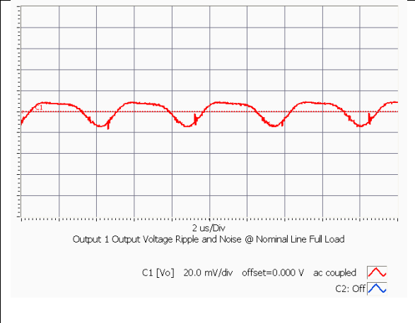
iEA4W004A120V-000 Typical Output Ripple at nominal input voltage and full load at Ta=25 degrees
