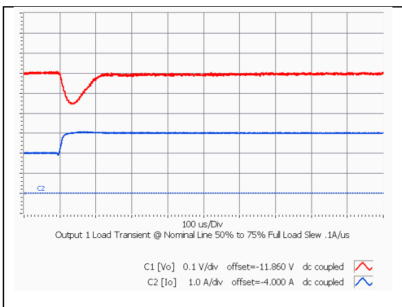
iEA4W004A120V-000 Typical Output voltage response to load step from 50% to 75% of full load with output current slew rate of 0.1A/uS and Cout = Cout,min.
