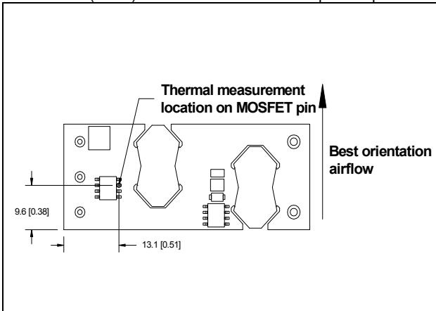
iEA4W004A120V-000 thermal measurement location – top view
