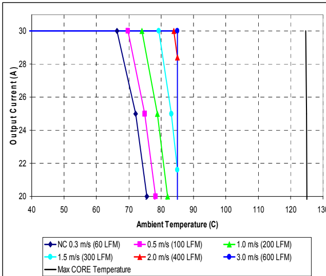
Maximum output current vs. ambient temperature at nominal input voltage with no base plate for airflow rates natural convection (0.3 m/s) to 3.0 m/s with airflow from pin 4 to pin 1.
