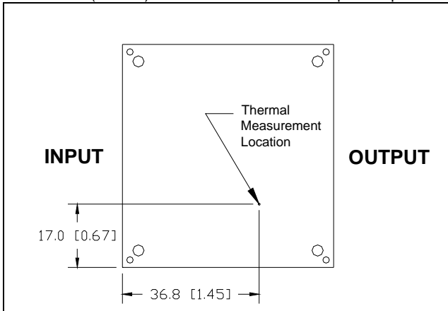
Thermal measurement location for module with base-plate: top view
