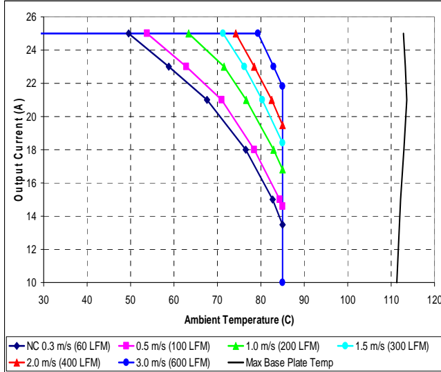
Maximum output current vs. ambient temperature at nominal input voltage with base plate for airflow rates natural convection (0.3 m/s) to 3.0 m/s with airflow from pin 4 to pin 1.
