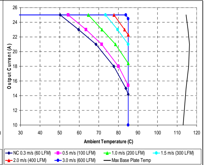
Maximum output current vs. ambient temperature at nominal input voltage with base plate for airflow rates natural convection (0.3m/s) to 3.0 m/s with airflow from pin 1 to pin 4.
