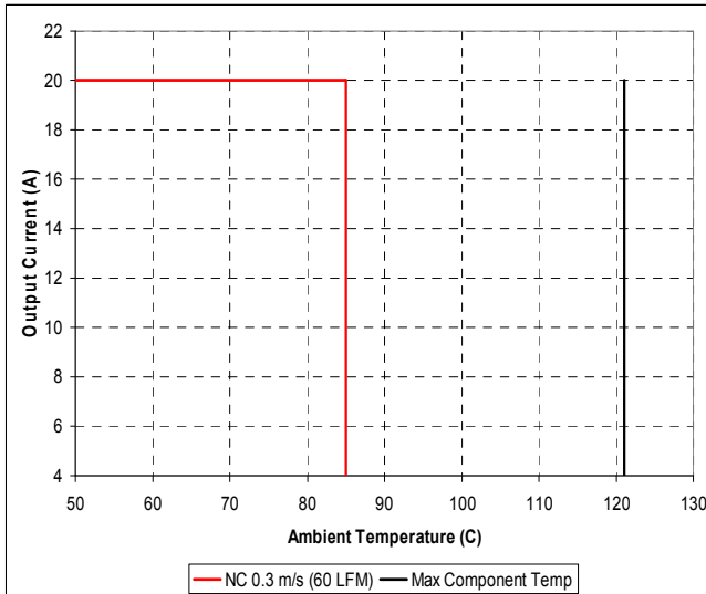
Maximum output current vs. ambient temperature at nominal input voltage for airflow rates natural convection (0.3m/s) and up with airflow from pin 4 to pin 1 (no base-plate).
