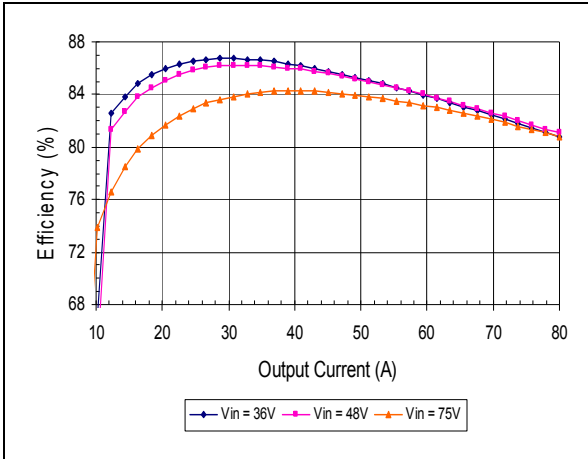
Typical Efficiency vs. Vin (test in socket, no baseplate)
