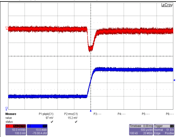
Load Transient Response. Load Step from 50% to 75% of Full Load with di/dt= 1A/uS. Ch. 1: Vo Ch. 2: Io
