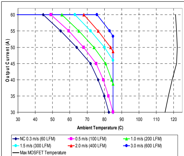
Maximum output current vs. ambient temperature at nominal input voltage for airflow rates natural convection (0.3m/s) to 3.0m/s with airflow from pin 4 to pin 1 (no base-plate).
