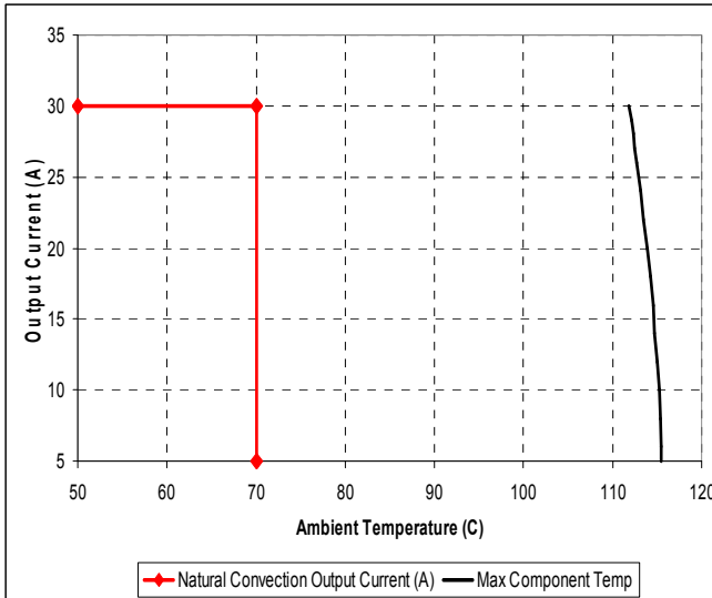
Maximum output current vs. ambient temperature at nominal input voltage for airflow rates natural convection (0.3m/s) and up with airflow from pin 4 to 1 (no base-plate).
