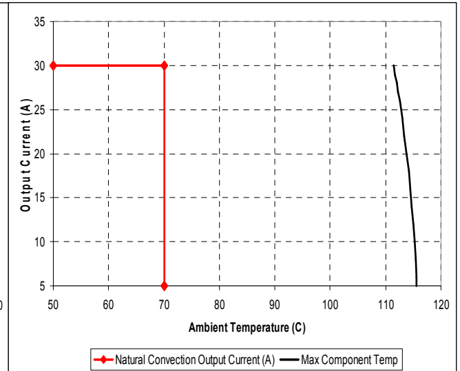
Maximum output current vs. ambient temperature at nominal input voltage for airflow rates natural convection (0.3m/s) and up with airflow from pin 1 to pin 4 (no base-plate).
