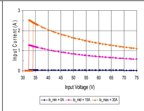
Typical Input Current vs. Input Voltage Characteristics
